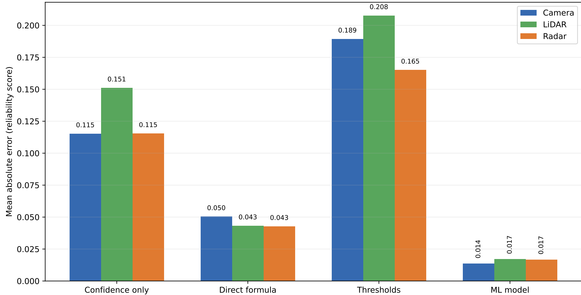
Graph 21. Sensor-reliability MAE by estimation method
