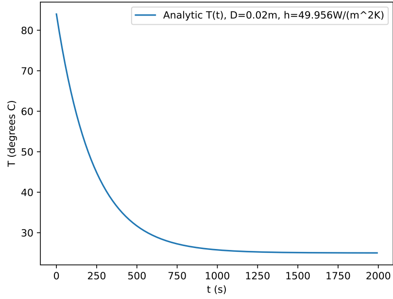
Figure 2: The lumped sum analytical solution of T(t) across times 0 \leq t \leq 1992.525 s.
