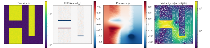
Fig. 3. A representative frame from our multiphase pressure-Poisson benchmark at N=16\,384 . Left : heterogeneous density p with 27\times contrast, separated by closed and partially-closed barriers (yellow). Middle : buoyancy-driven right-hand side b = -\partial_y p , concentrated on horizontal density interfaces. Right : recovered pressure p with velocity -\nabla p/\rho overlaid.
