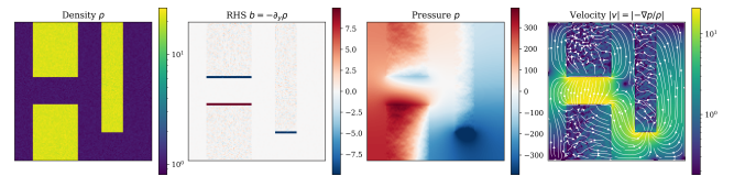
Fig. 3. A representative frame from our multiphase pressure-Poisson benchmark at N = 16\,384 . Left : heterogeneous density p with 27\times contrast, separated by closed and partially-closed barriers (yellow). Middle : buoyancy-driven right-hand side b = -\partial_y p , concentrated on horizontal density interfaces. Right : recovered pressure p with velocity -\nabla p/p overlaid.
