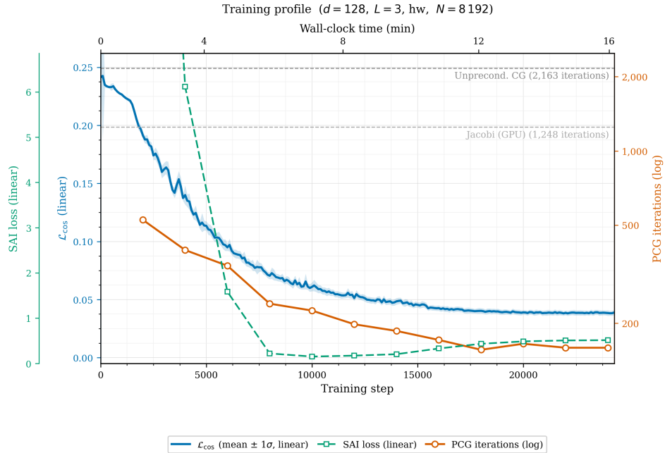
Fig. 4. Training profile of the configuration used in Table 2 ( N=8192 , d=128 , n_l=3 , highways). Blue: \mathcal{L}_{\cos} on the training set (mean \pm 1\sigma , last 100 steps). Green dashed: SAI loss [Yang et al. 2025] computed on a held-out validation frame at the same checkpoints ( not used for training). Orange: PCG iteration count to \text{rtol}=10^{-8} on that frame, log scale. Top axis: wall-clock minutes. Horizontal grey lines: unpreconditioned CG and Jacobi GPU baselines.
