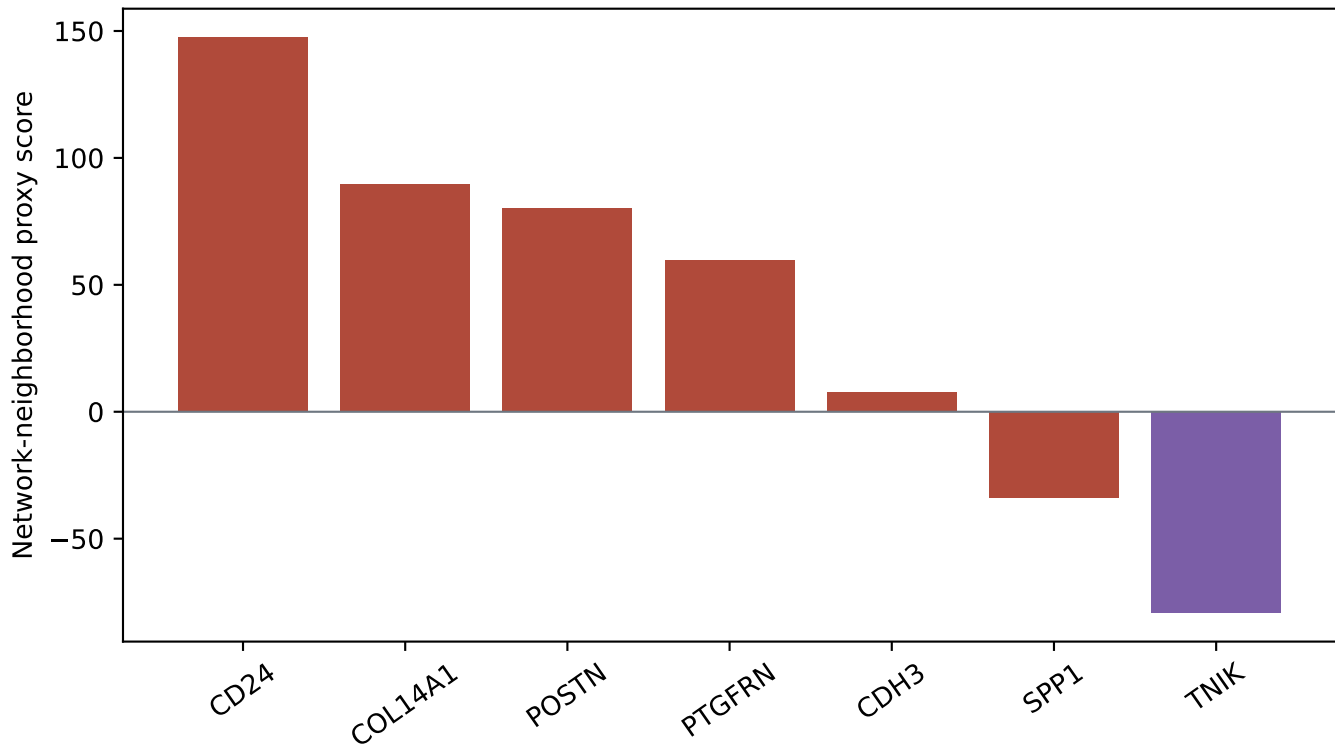
Coexpression-neighborhood proxy prioritizes candidates
