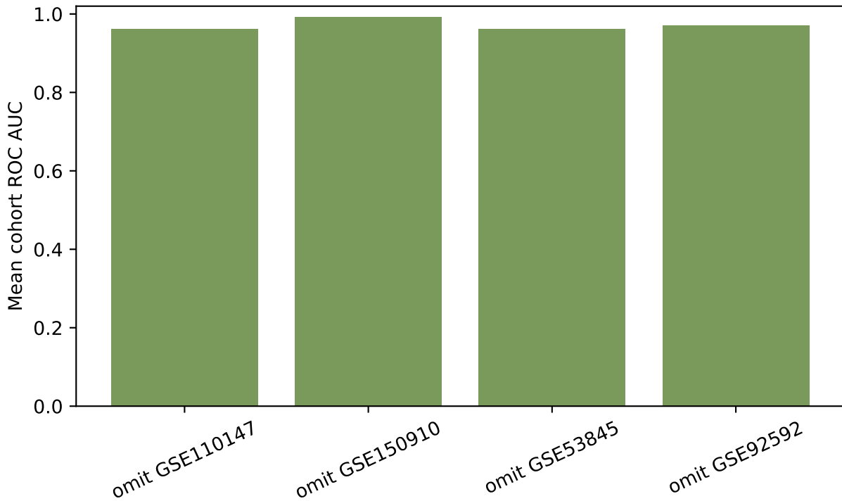
Leave-one-validation-cohort sensitivity
