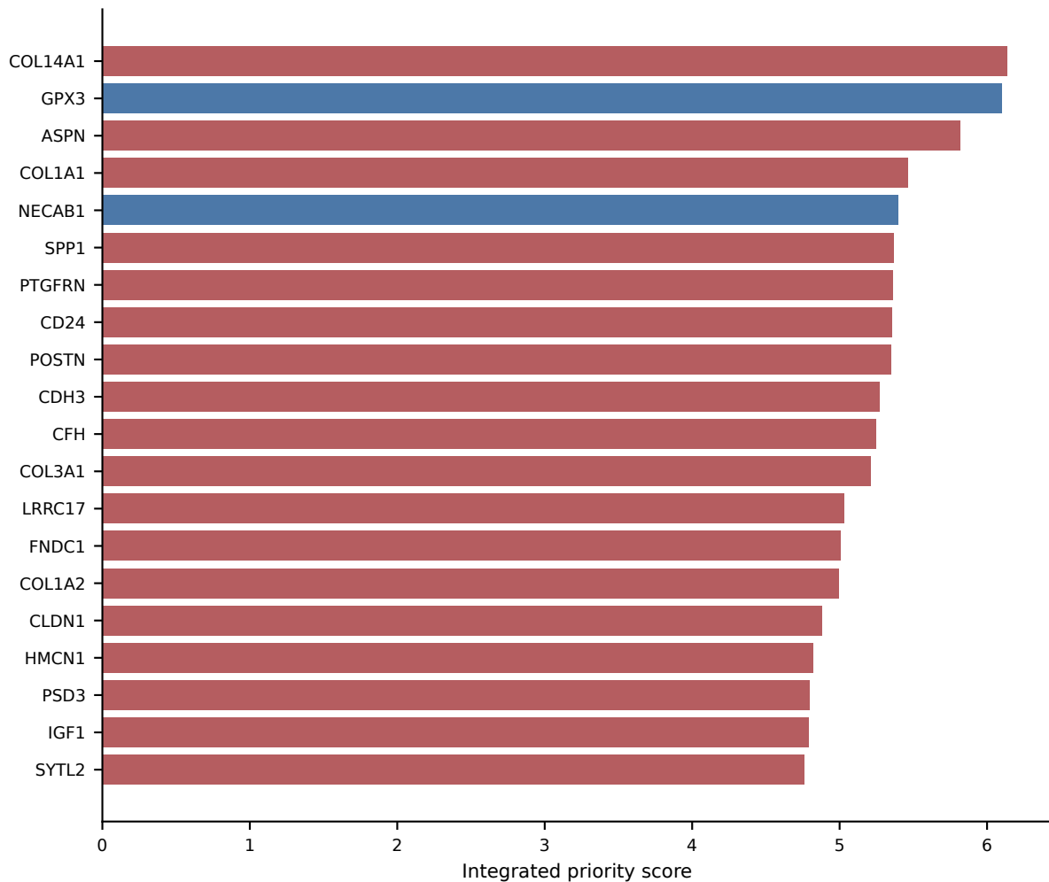
Top integrated oligonucleotide-candidate targets
