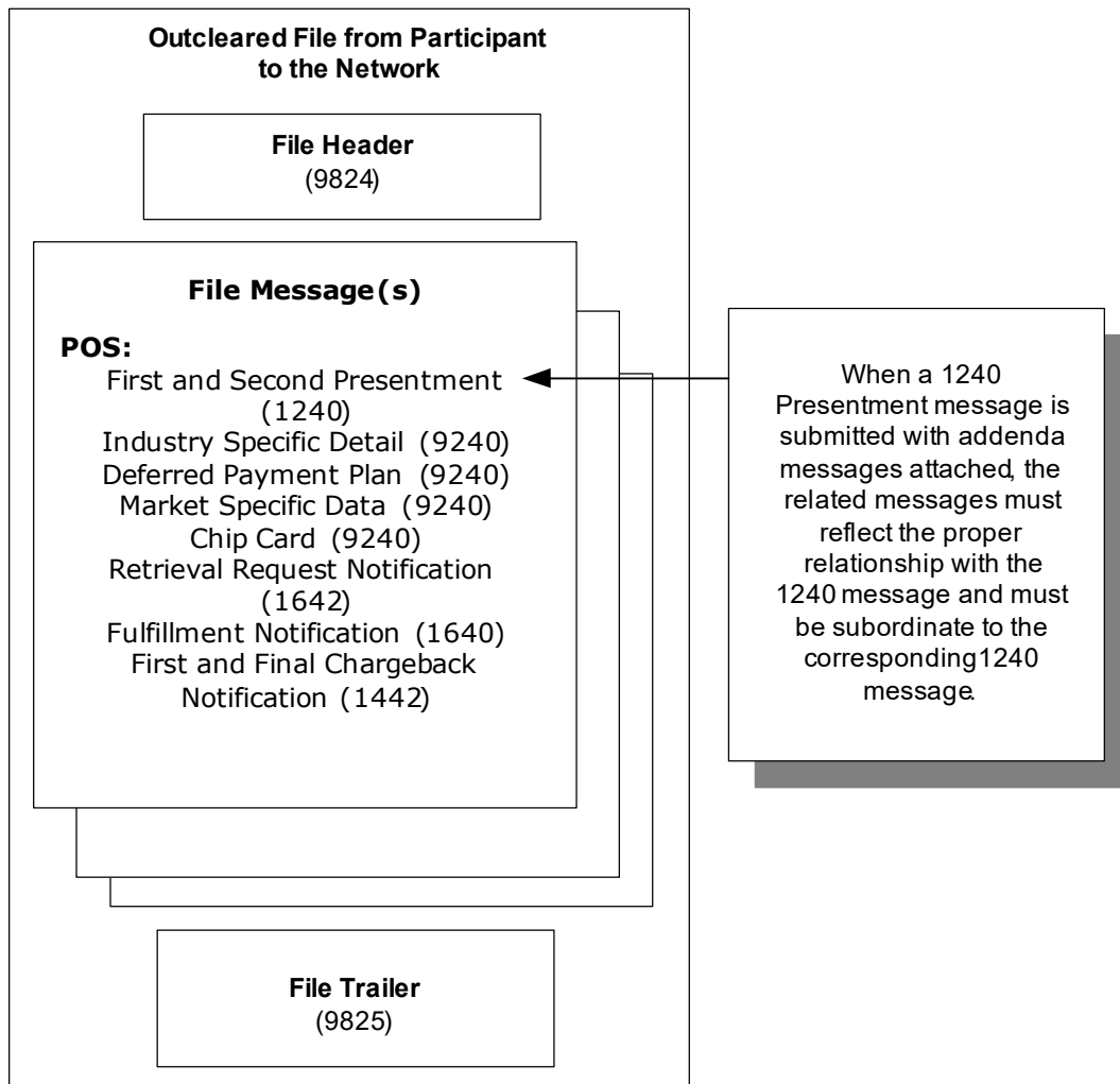
Figure 2-3. Example of Outcleared Financial Messages
