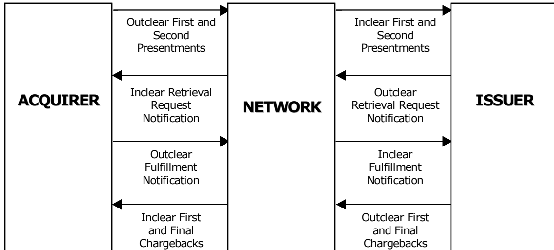
Figure 2-1. Flow Between Acquirer and Issuer through the Network
