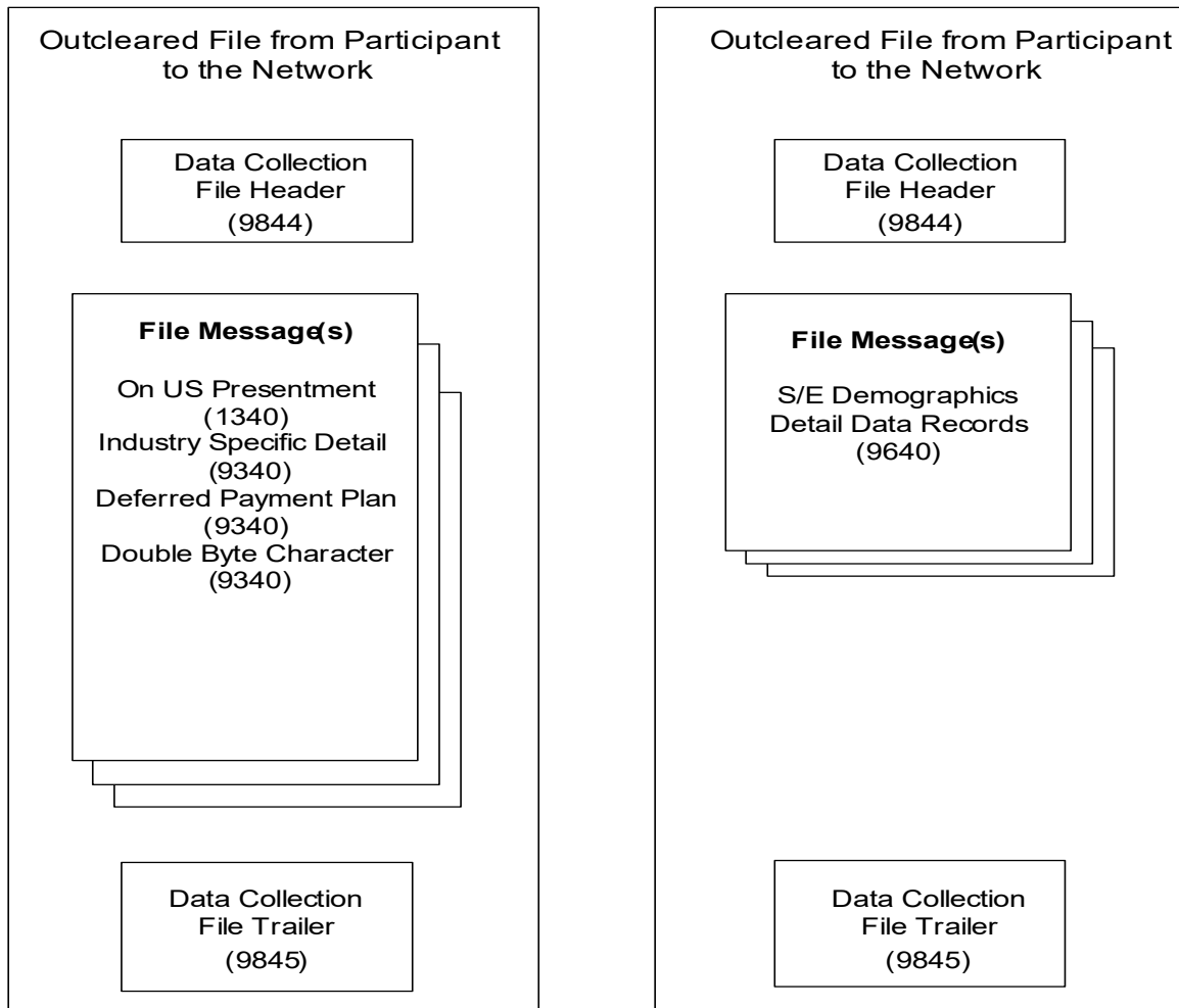
Figure 5-2. Example of Outcleared Data Collection Messages
