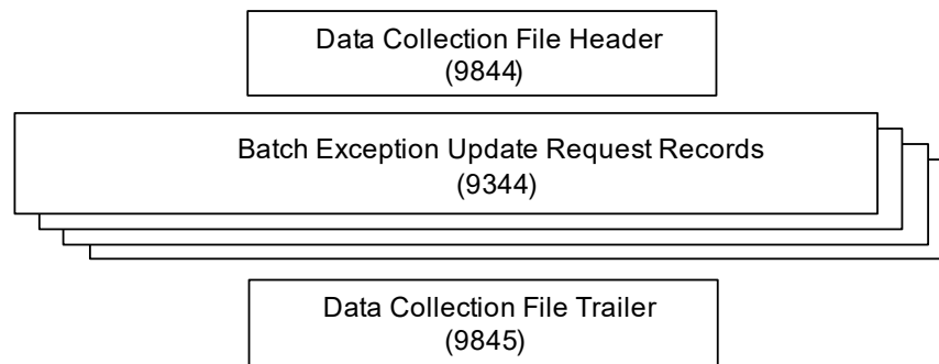
Figure 5-5. Batch Exception Update Request File Structure
