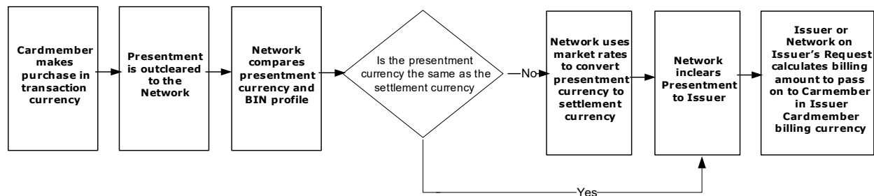
Figure 2-6. Flow of Multi-Currency Presentment
