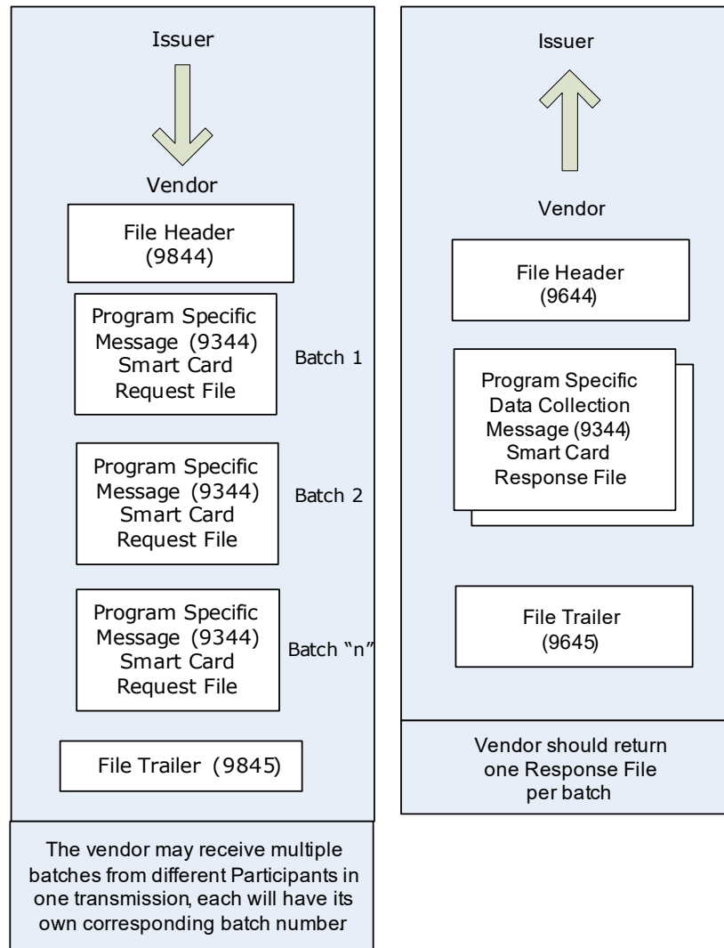
Figure 5-4. Chip Card Request and Response File Structure
