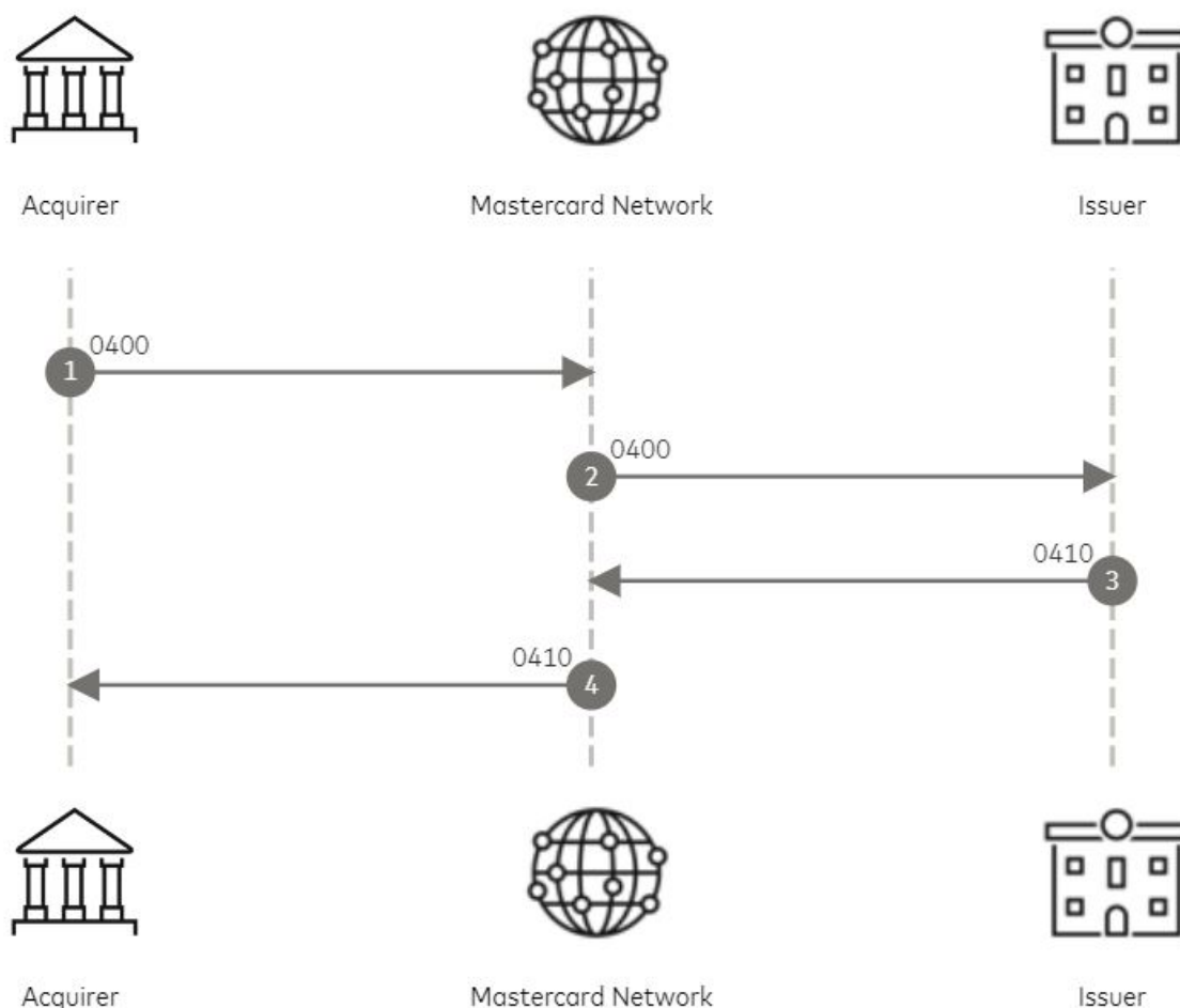
Figure 14: Standard Reversal Request flow
