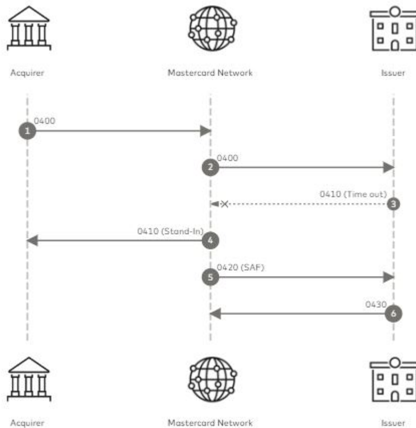
Figure 15: Reversal request no response from issuer or not within time limit flow
