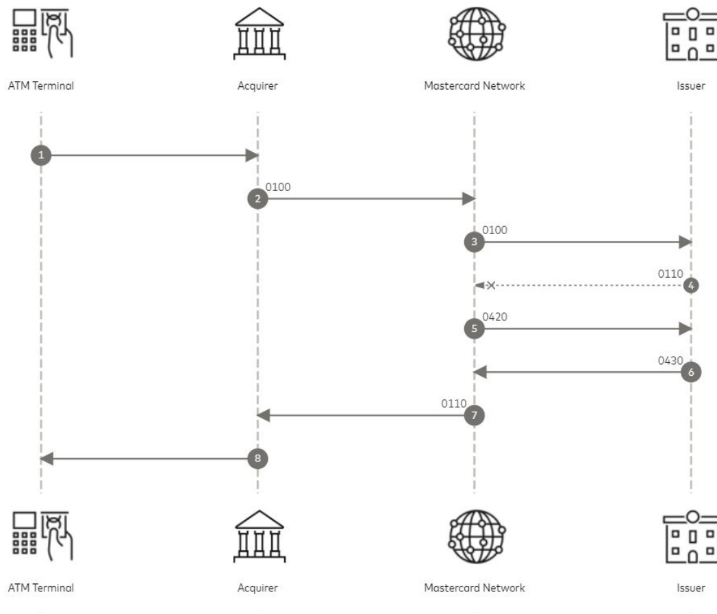
Figure 5: PIN-management Response not received from issuer flow
