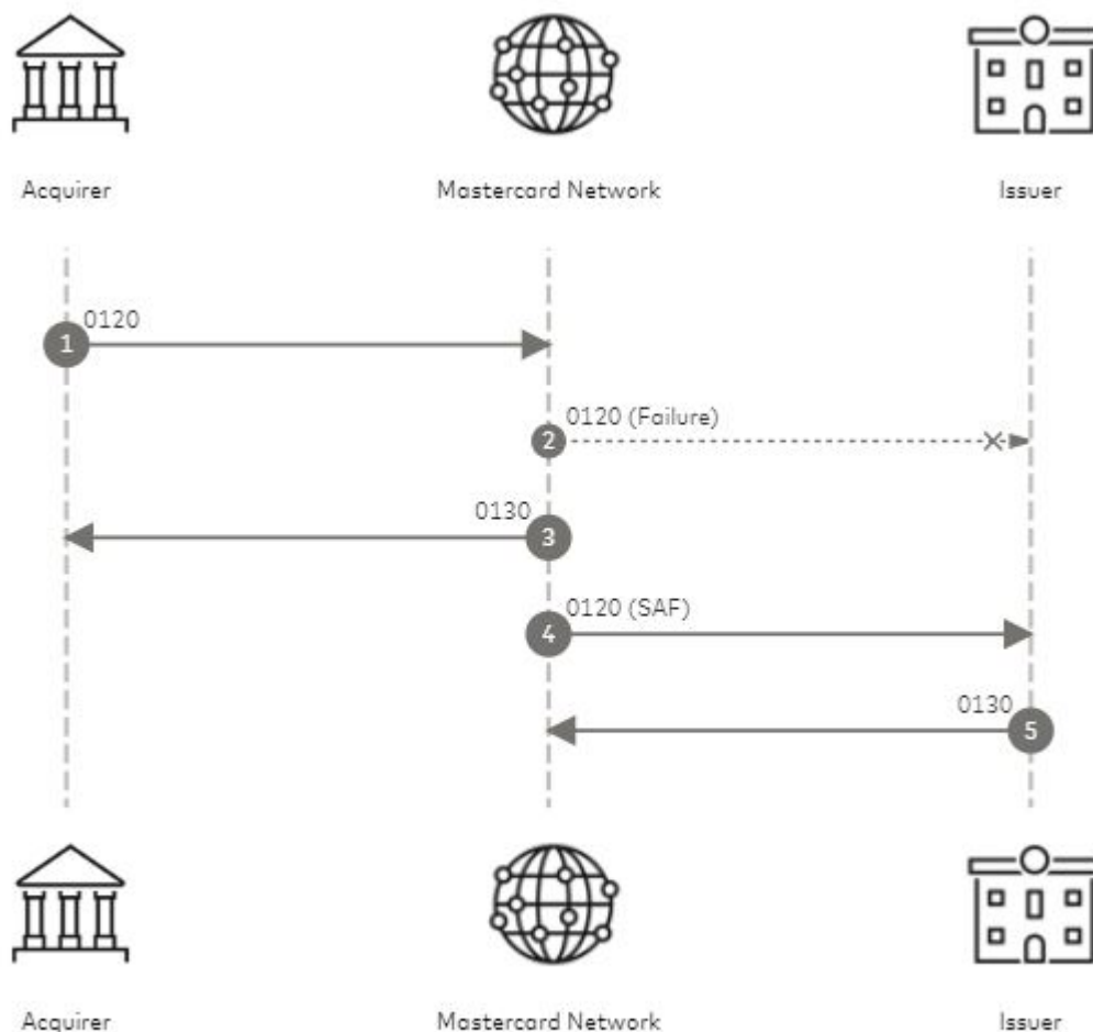
Figure 9: Acquirer-generated advice message, issuer not available flow
