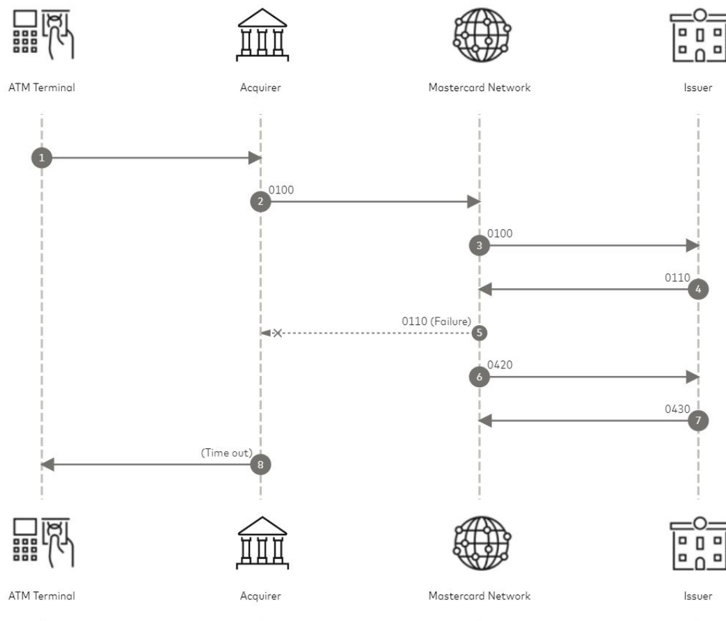
Figure 7: Chip-PIN Management Response cannot be delivered to the acquirer flow
