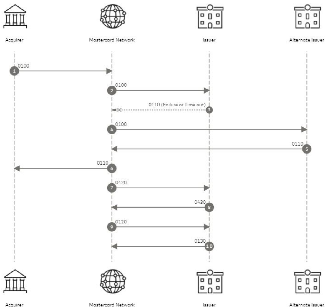
Figure 11: Primary issuer times out flow
