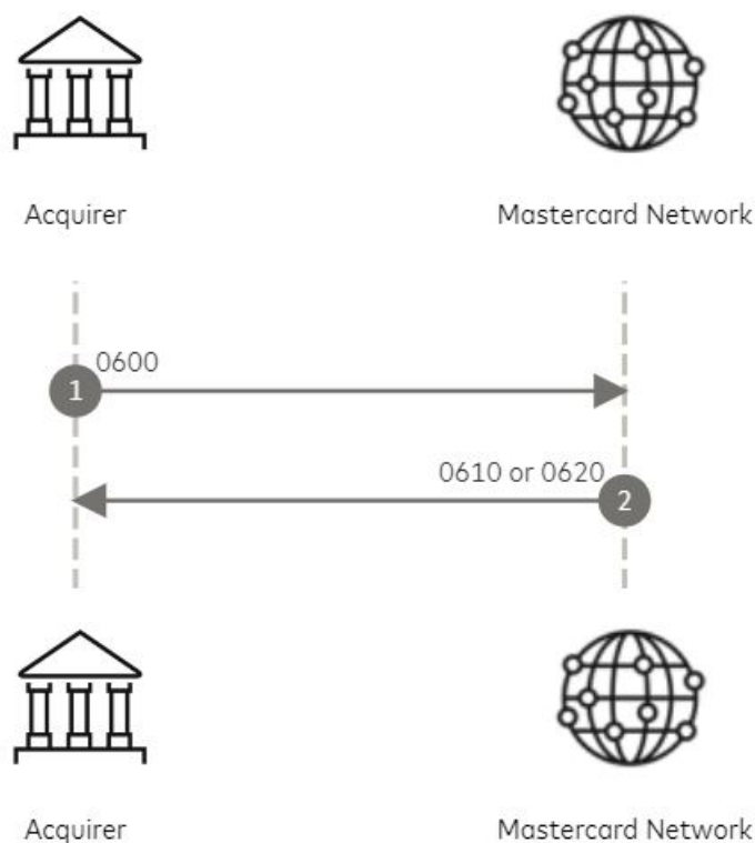
Figure 20: Acquirer-edit Failure flow
