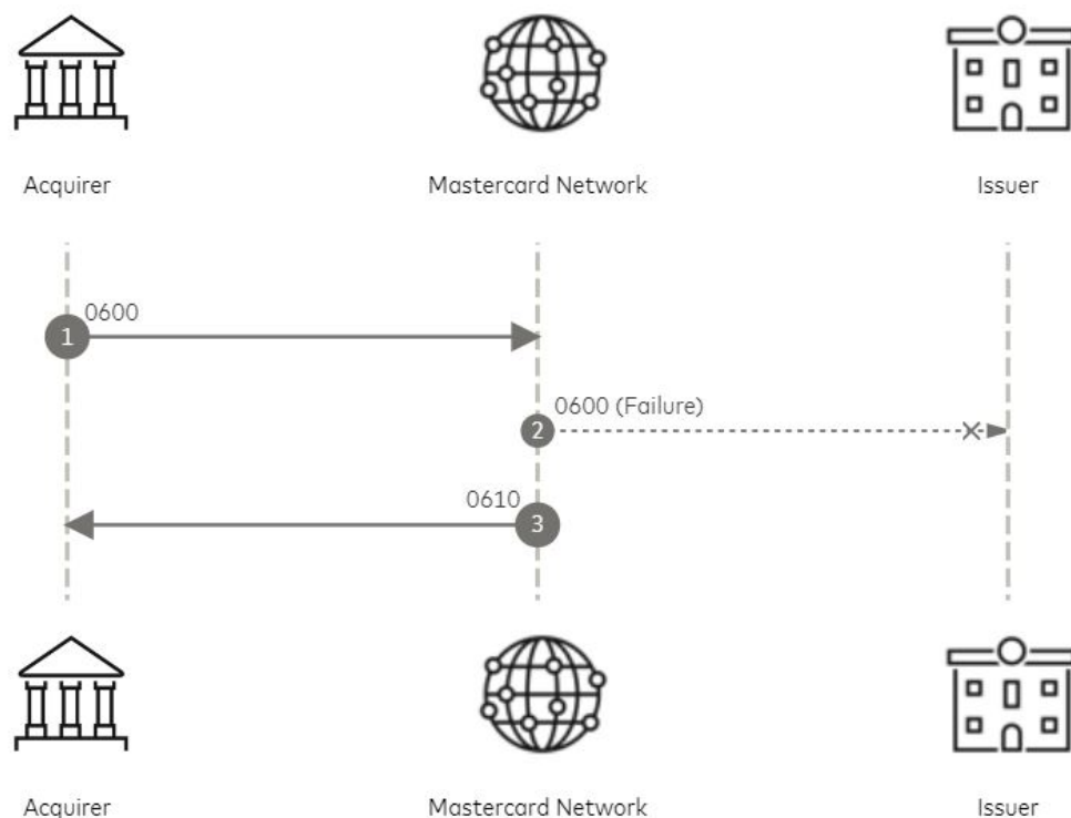
Figure 21: Communication Failure at issuer flow
