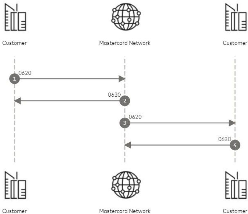
Figure 25: Standard Administrative Advice flow
