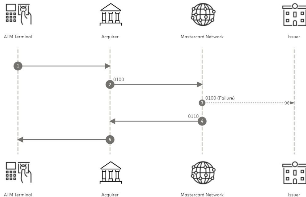
Figure 4: Chip-PIN Management Request unable to connect to issuer flow
