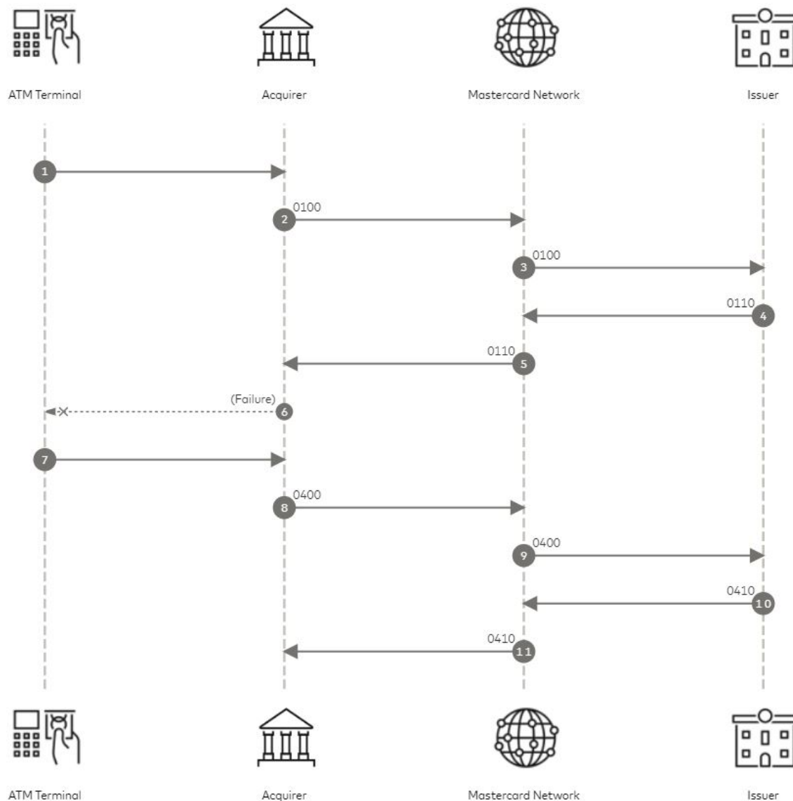
Figure 3: Chip-PIN Management Update cannot be transmitted or applied to chip card flow
