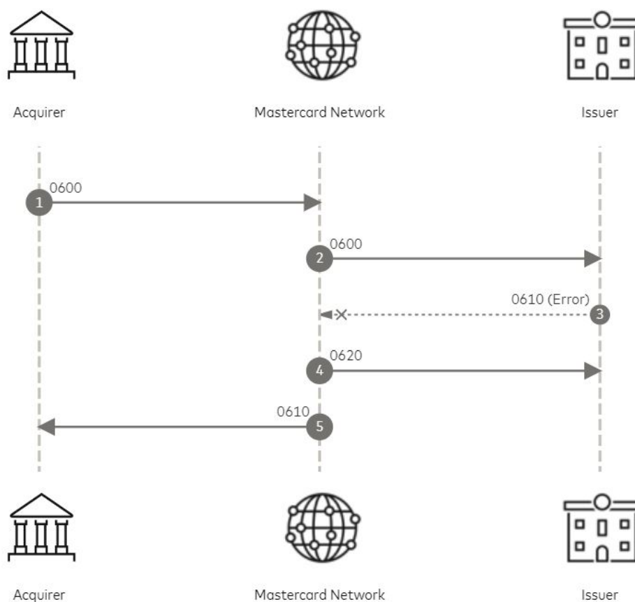
Figure 24: Issuer-edit Failure flow
