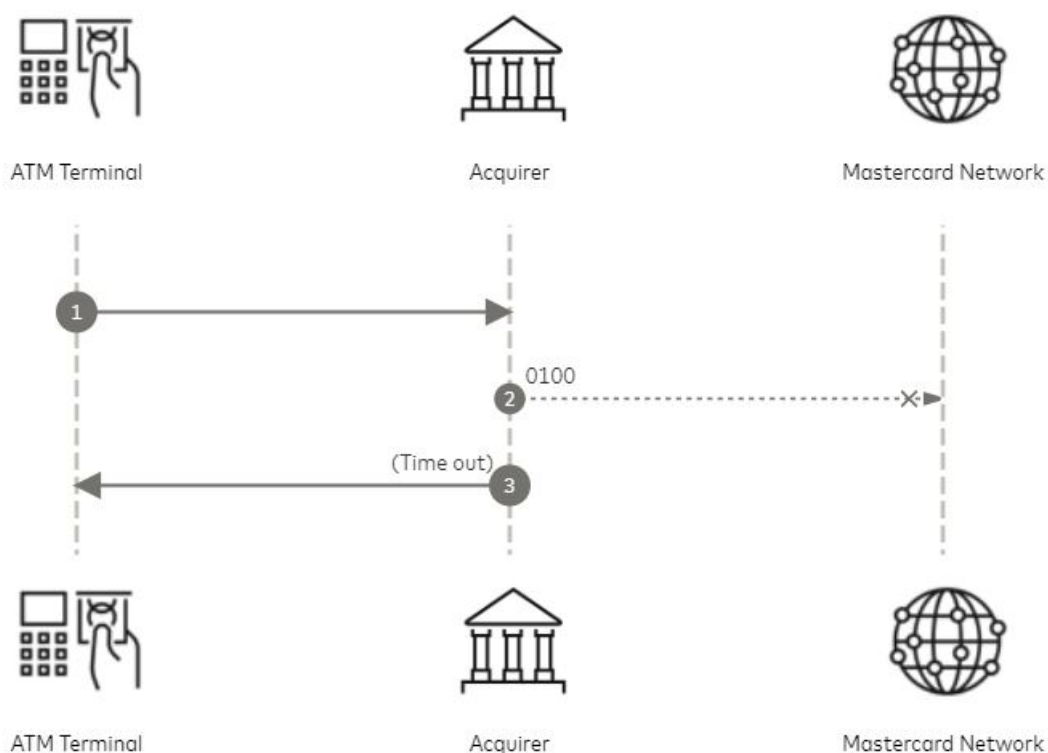
Figure 6: Chip-PIN Management Request failure from acquirer flow
