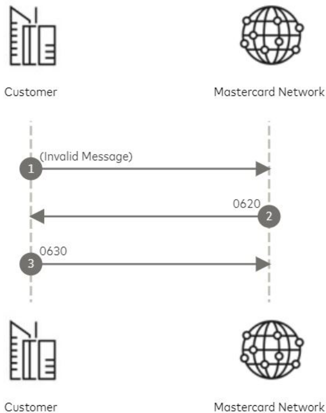
Figure 26: Failure scenario: Administrative Advice for invalid message flow
