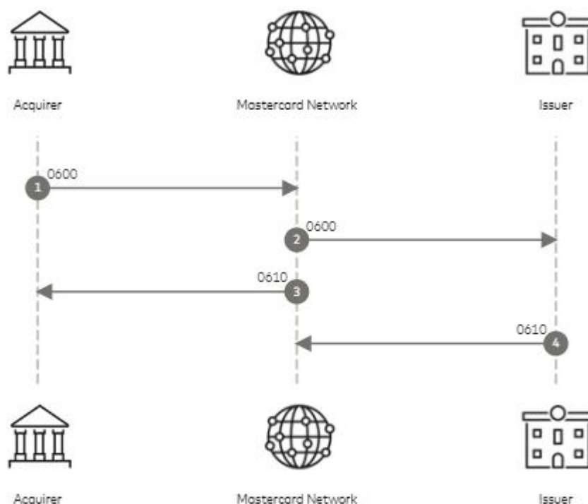
Figure 23: Late or no issuer response flow
