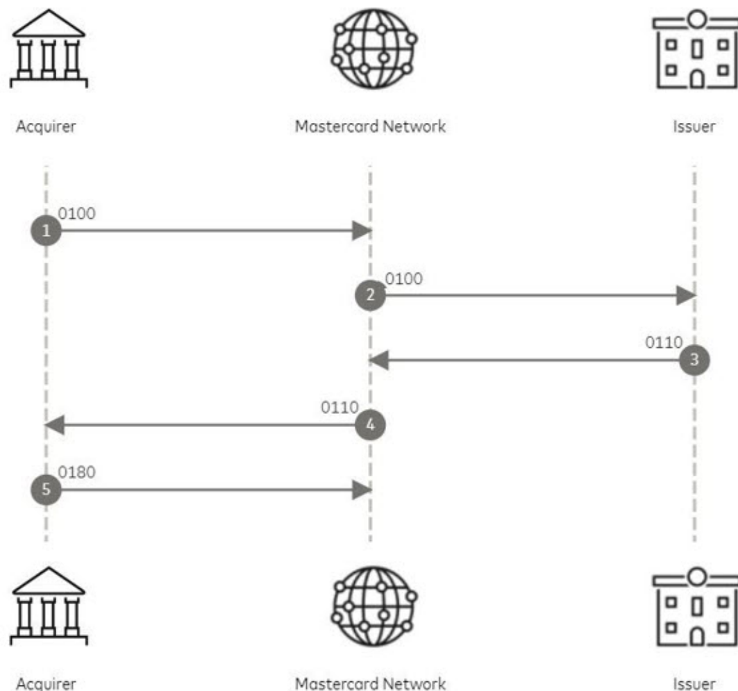
Figure 10: Acquirer Response Acknowledgment flow
