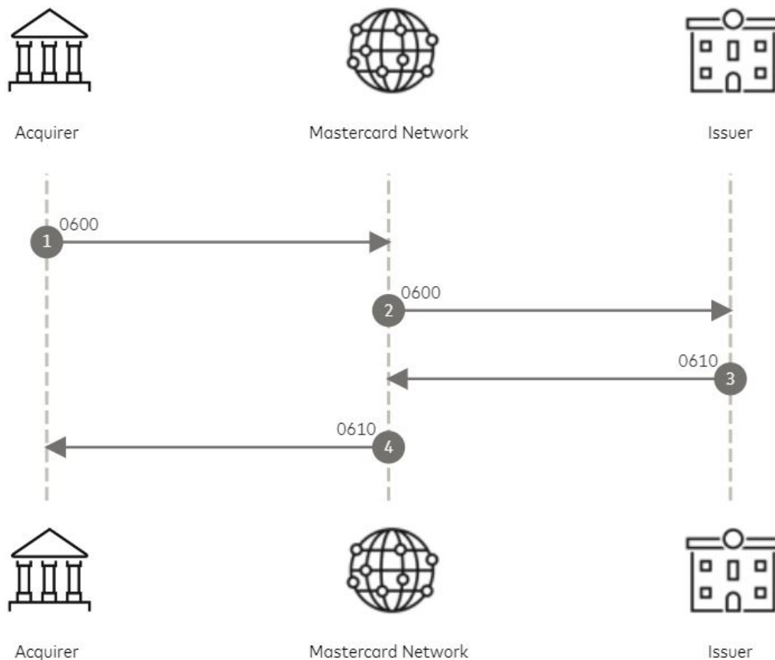
Figure 19: Standard Administrative request flow
