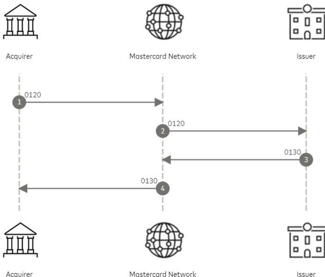
Figure 8: Acquirer-generated authorization advice message standard flow
