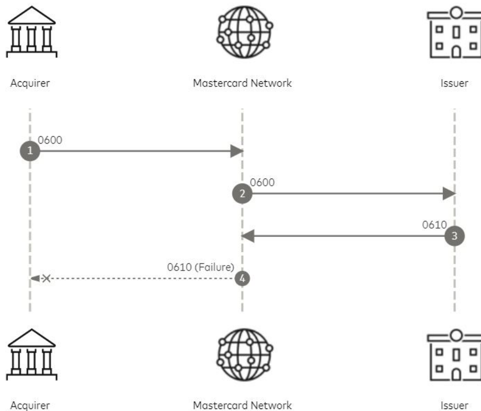
Figure 22: Communication Failure at acquirer flow
