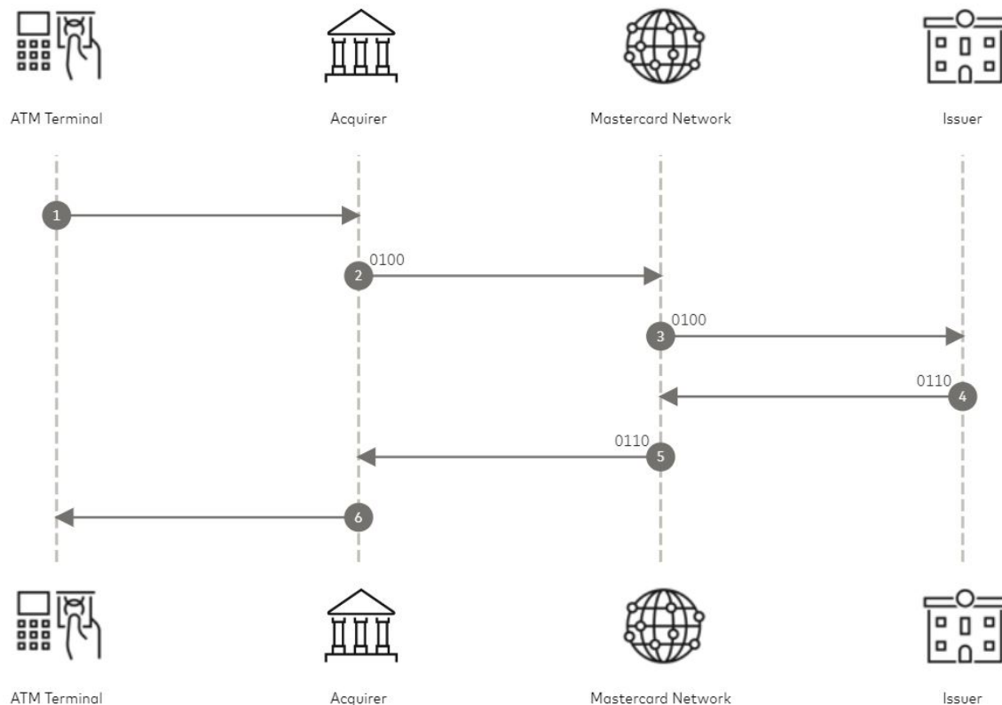
Figure 2: Standard Chip-PIN Management request flow
