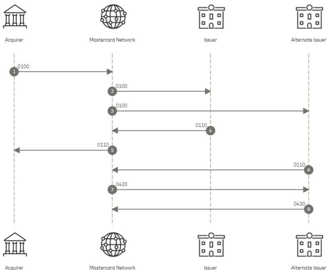
Figure 12: Primary issuer responds after time limit and primary issuer response received first flow
