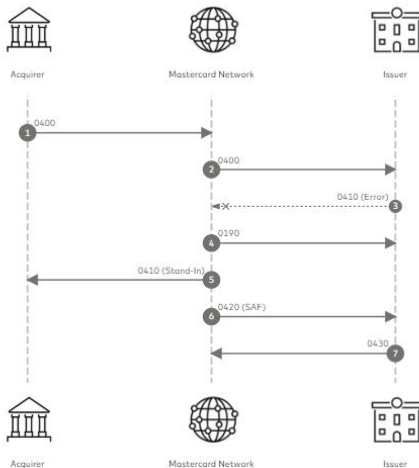
Figure 17: Reversal request response from issuer contains errors flow
