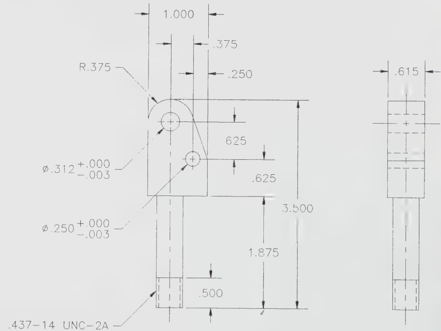
⑭ PUMP PIVOT SUPPORT
