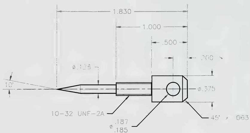
(29) NEEDLE VALVE
