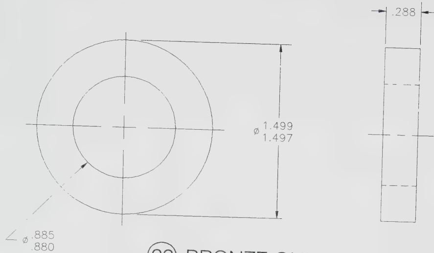
(22) BRONZE GUIDE
