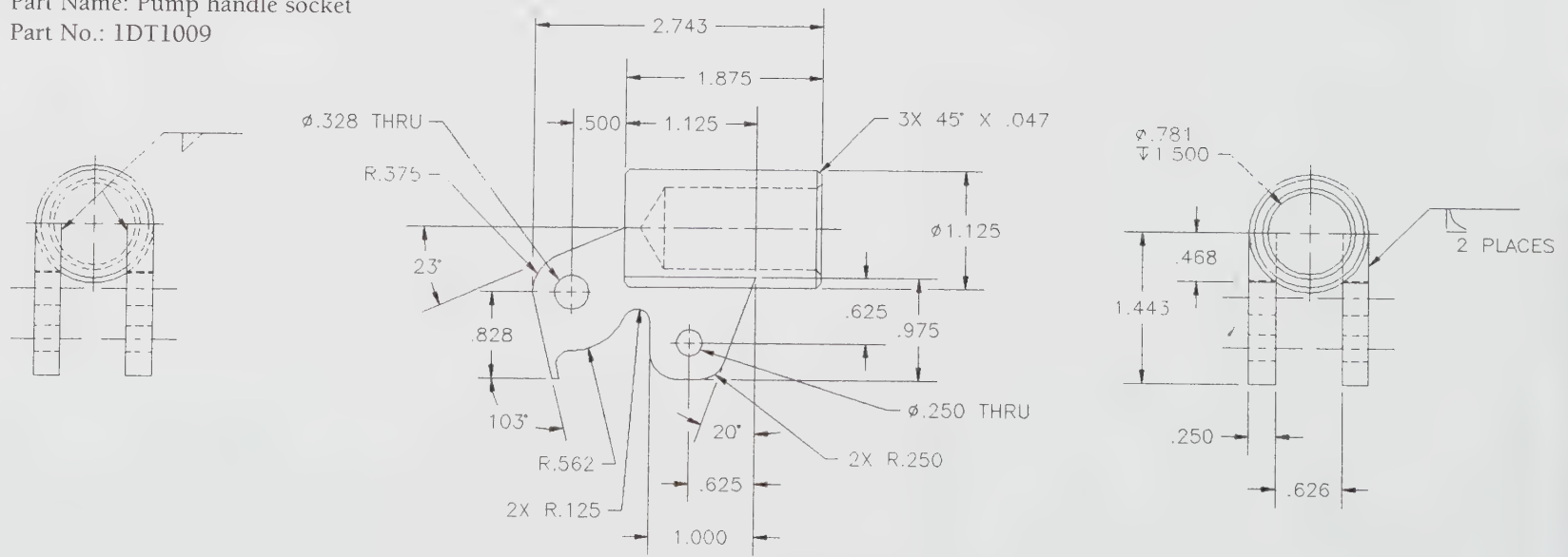
⑨ PUMP HANDLE SOCKET
