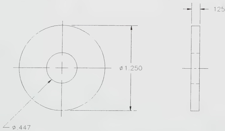
⑳ PISTON WASHER
