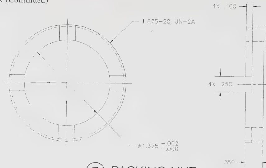
⑦ PACKING NUT
