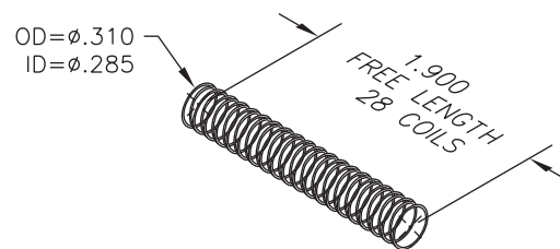
12 PSI CONTROL SPRING
