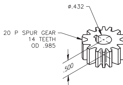
15 IDLER GEAR (FEED)
