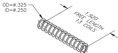
10 PLUNGER SPRING
