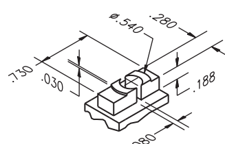
VIEW A ④ SCREW ADJUSTER
