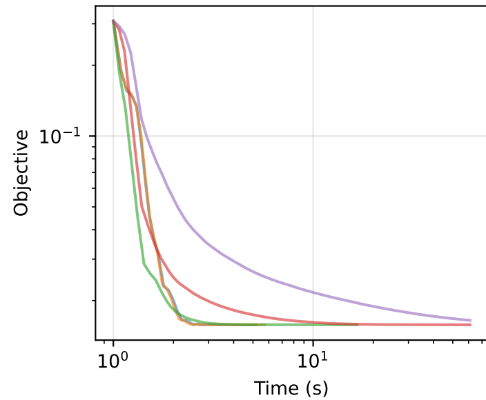
Objective value
