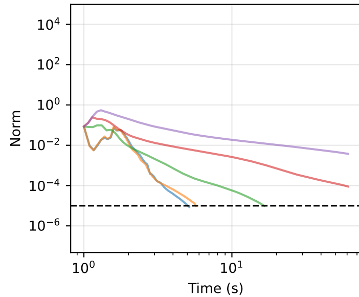
Stationarity
