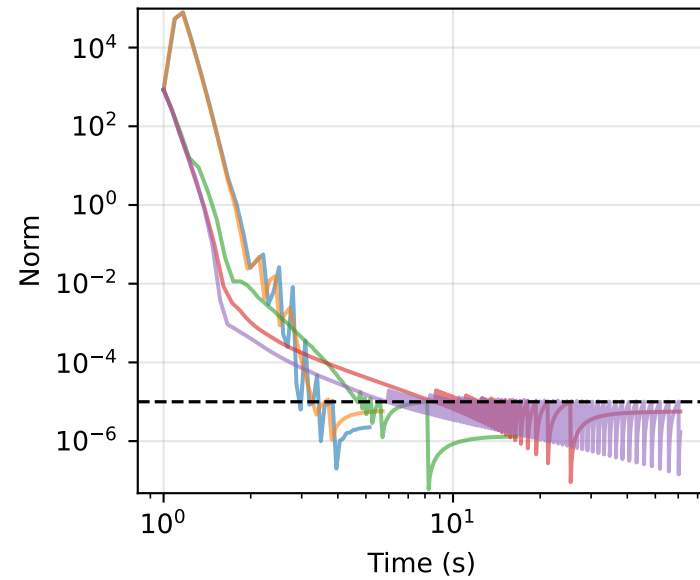
Constraint norm
