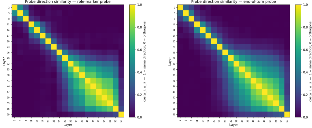
Figure 31: Probe-direction cosine across layers, within each token position. Left: role-marker; right: end-of-turn. Both positions show the same block structure: early layers (L2–L17) and late layers (L29–L59) form two loosely-aligned families, with the late block mutually aligned at cosine \geq 0.5 and internally tightly aligned ( \geq 0.8 ) among adjacent layers. Early layers are close to orthogonal to the late block.
