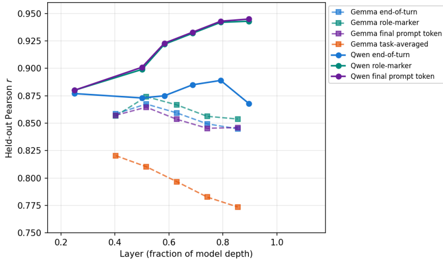
Figure 35: Held-out Pearson r by layer and token position, both models. Qwen-3.5-122B (solid) and Gemma-3-27B (dashed) on a shared layer-depth axis (fraction of total layers). Ridge probes trained on the legacy 10k pool, evaluated on an independent 4k measurement run. Within each model, the three turn-boundary positions cluster tightly; Gemma’s task-averaged position is visibly lower. Qwen was not swept at the task-averaged position.
