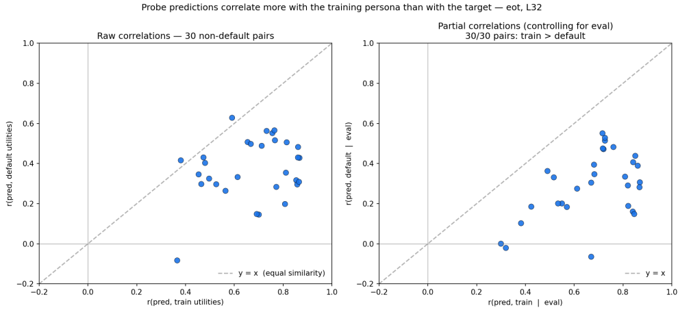
Figure 25: Probe prediction pattern vs train and default utilities. For each of the 30 non-default (T, E) ordered pairs, x = r(\hat{u}, u_T) , y = r(\hat{u}, u_{\text{def}}) . Left : raw Pearson r ; 28/30 sit on the train-favouring side of y = x . Right : partial correlations after regressing out the eval utilities u_E ; 30/30 sit on the train-favouring side. Mean partial r(\hat{u}, u_T | u_E) = +0.672 , partial r(\hat{u}, u_{\text{def}} | u_E) = +0.293 .
