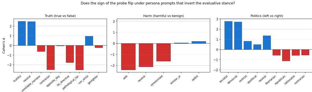
Figure 36: Cohen’s d under every persona prompt tested. One panel per domain. Bars positive = first-listed condition scores higher (true; harmful; left). Truth: lying-persona prompts flip the sign from +2.5 to -2.53. Harm: evil-persona prompts collapse |d| toward zero. Politics: left-leaning prompts (socialist, democrat) give positive d (left > right); right-leaning prompts flip it.
