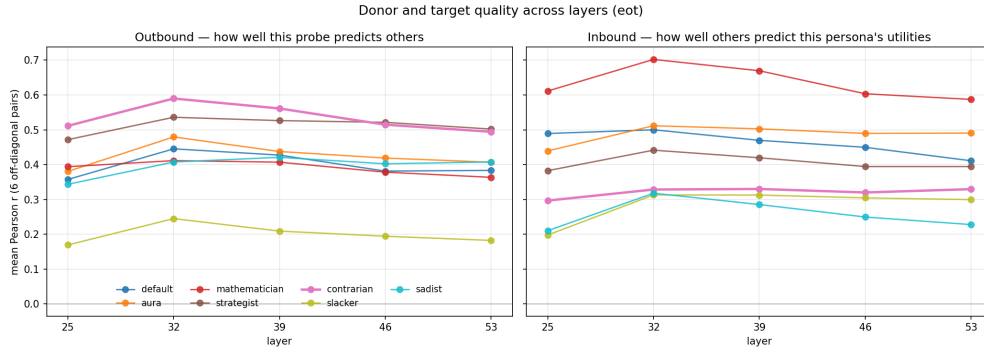
Figure 22: Donor and target quality across layers. Outbound mean r (left) and inbound mean r (right) vs layer, one line per persona. Contrarian (bold) is the best donor at every layer; slacker is the worst.
