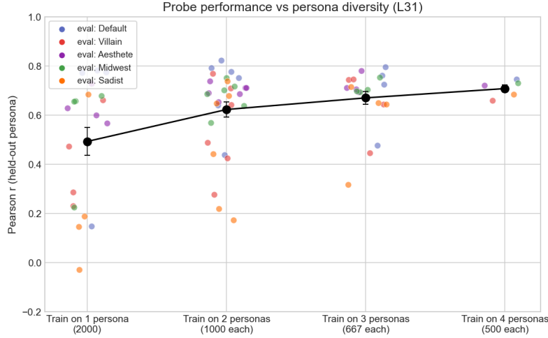
Figure 27: Persona-diversity ablation. Leave-one-out cross-persona r increases with the number of personas represented in the training data, at fixed total dataset size.
