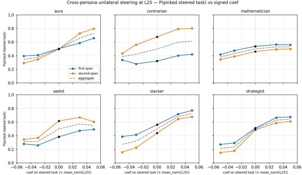
Figure 9: Cross-persona unilateral steering at layer 25. P(\text{picked steered task}) against signed coefficient on the steered task’s tokens, per persona. Blue = coefficient applied to the first-presented span, orange = to the second-presented span, gray dashed = the two averaged (removes position bias). Black dots at c = 0 are empirical no-steering baselines (600 generations per persona via API; see text).
