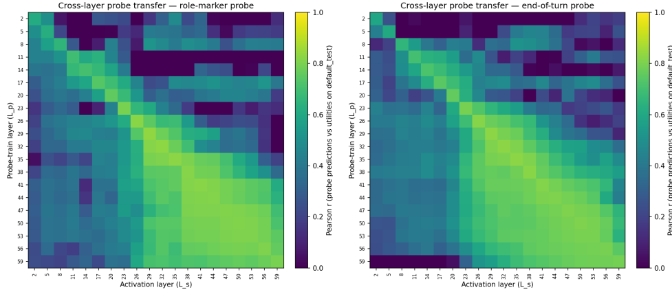
Figure 33: Cross-layer probe transfer. Each cell: Pearson r between predictions of the probe trained at layer L_p (row) evaluated on activations at layer L_s (column), versus held-out utilities. The diagonal is each probe’s native performance (equivalent to Fig. 30). Off-diagonal cells in the mid-to-late block stay near the diagonal value, reflecting the tight cosine alignment seen in Fig. 31. Early-layer probes (top rows) transfer poorly to late activations and vice versa.
