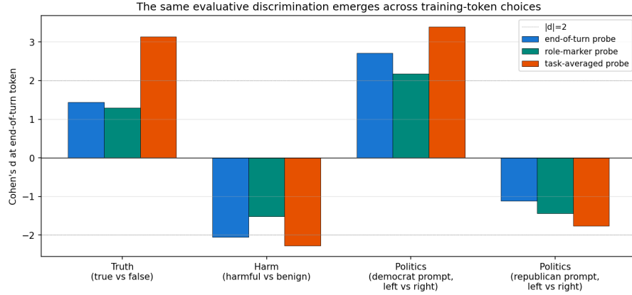
Figure 37: Same discrimination across training-token choices. Cohen’s d at the end-of-turn token on truth / harm / politics evaluative pairs, under three ridge probes trained at different positions (end-of-turn, role-marker, task-averaged; see App. G). Positive = first-listed class scores higher (true; harmful; left). All three probes agree in sign; democrat-prompt politics is positive, republican-prompt politics flips negative.
