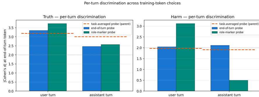
Figure 38: Per-turn discrimination. |d| split by user vs assistant turn. The end-of-turn probe is turn-stable; the role-marker probe collapses on assistant-turn harm because of a structural-position artefact. Dashed horizontal: the task-averaged probe pooled across turns.
