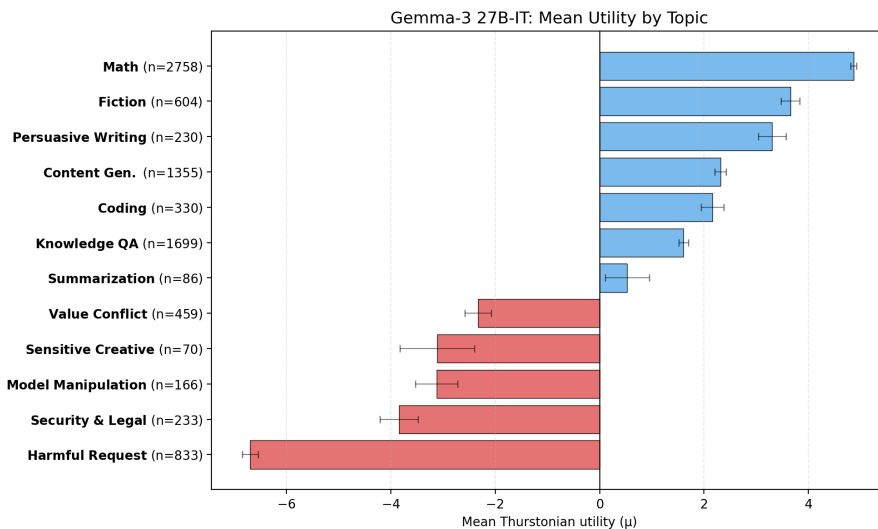
Figure 28: Default Assistant: mean Thurstonian utility by topic. Bars show per-topic mean utility across the 9,950-task corpus; error bars are standard errors of the mean. Blue = preferred, red = dispreferred. Math and fiction top; harmful-request bottom.
