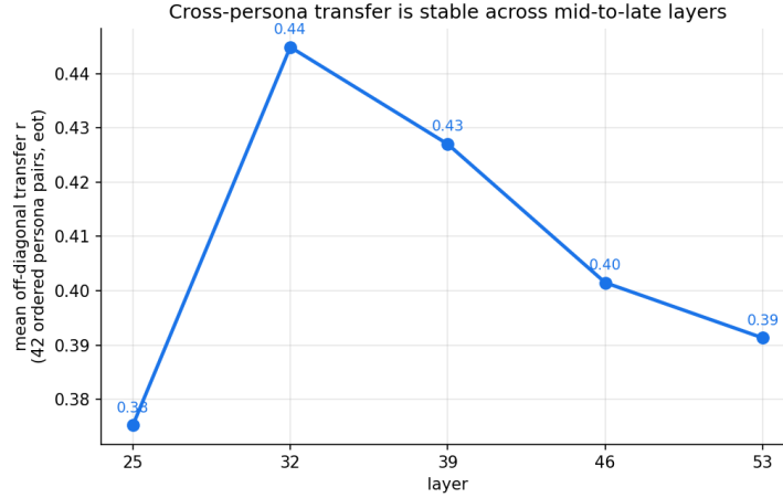
Figure 23: Mean off-diagonal transfer r across layers (eot). Average over all 42 ordered (train, eval) persona pairs. The cross-persona transfer signal is approximately layer-invariant in the L25–L53 range.
