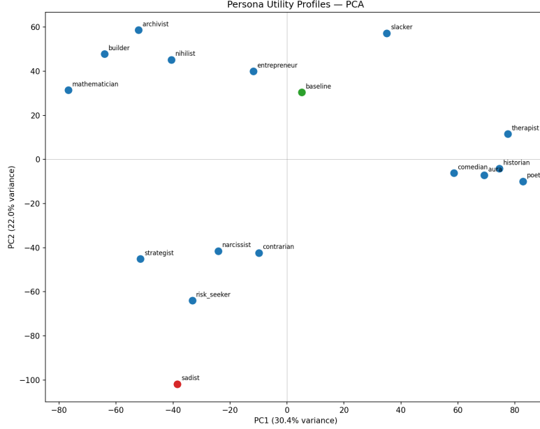
Figure 21: PCA of the 16-persona utility sweep. Each point is a persona’s Thurstonian utility profile on the 500-task stratified sample, projected onto the first two principal components (52% of variance). Three clusters emerge: structured/analytical (left), creative/humanistic (right), dark/oppositional (bottom-centre). Sadist (red) is the only persona whose utility anti-correlates with the no-system-prompt baseline (green). The final six-persona set takes one representative per cluster plus sadist, slacker, and aura.
