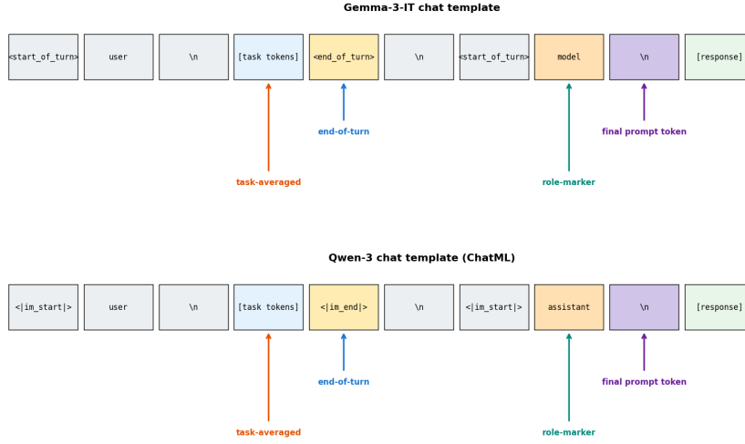
Figure 34: Turn-boundary positions in Gemma-3-IT and Qwen-3 chat templates. Each row shows the tokenisation of a typical user turn just before the model generates. Coloured arrows mark the four positions considered throughout this paper. The two templates use different special tokens but align one-for-one at the turn boundary.
