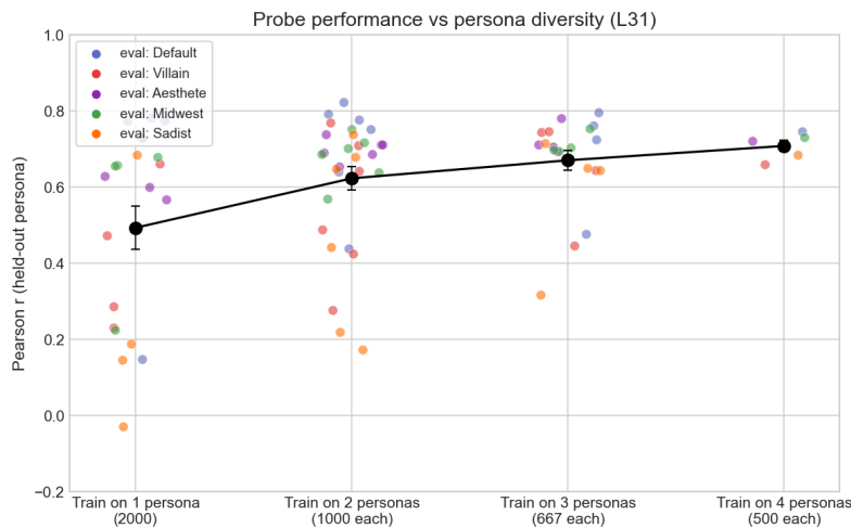
Figure 33: Persona-diversity ablation. Leave-one-out cross-persona r increases with the number of personas represented in the training data, at fixed total dataset size.
