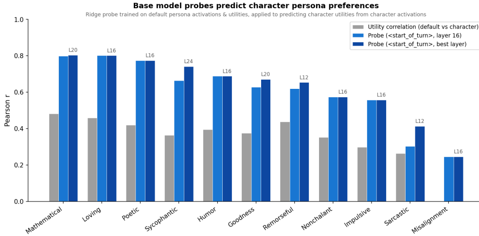
Figure 34: Base-model probe predicts character-fine-tuned persona preferences. Grey: raw correlation between base-model utilities and each character’s utilities. Light blue: probe at <start_of_turn> _ 2 , layer 16. Dark blue: same selector, best layer per persona (layer annotated). The probe beats the utility-correlation baseline on 10/11 personas. Misalignment is the hardest case: its raw utilities anti-correlate with the base model ( r = -0.14 ), yet the probe still recovers a positive correlation ( r = 0.25 ) — the largest absolute gain of any persona.
