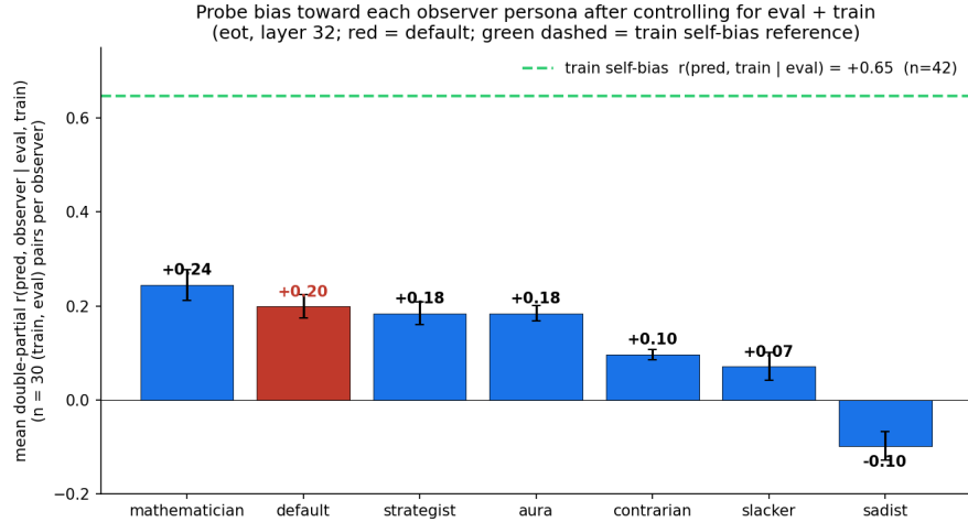
Figure 32: Probe bias toward each observer persona after controlling for eval and train. Mean double-partial r(\hat{u}, u_X \mid u_E, u_T) across 30 ordered (T, E) pairs per observer; error bars are SEM. Green dashed line: train self-bias r(\hat{u}, u_T \mid u_E) = +0.65 (42 pairs). Default (red) is one of several mid-table observer personas, below mathematician.
