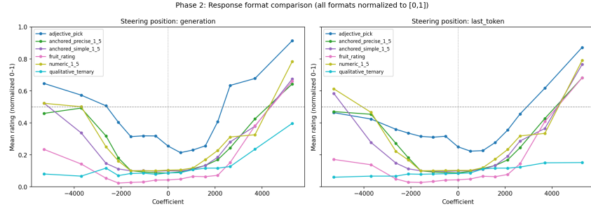
Figure 36: Normalised steerability by response format. All six formats yield significant dose-response. Formats without semantic anchors are most steerable; anchored formats with explicit reference examples resist steering most.
