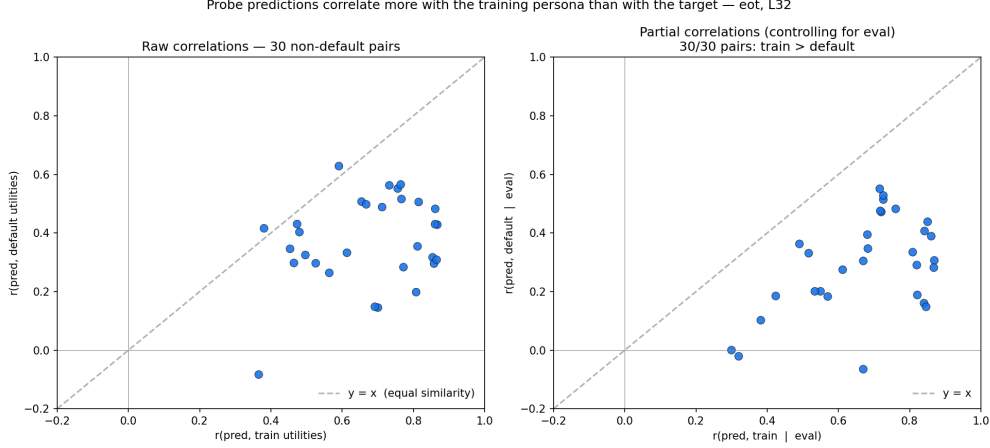
Figure 31: Probe prediction pattern vs train and default utilities. For each of the 30 non-default (T, E) ordered pairs, x = r(\hat{u}, u_T) , y = r(\hat{u}, u_{\text{def}}) . Left : raw Pearson r ; 28/30 sit on the train-favouring side of y = x . Right : partial correlations after regressing out the eval utilities u_E ; 30/30 sit on the train-favouring side. Mean partial r(\hat{u}, u_T | u_E) = +0.67 , partial r(\hat{u}, u_{\text{def}} | u_E) = +0.29 .
