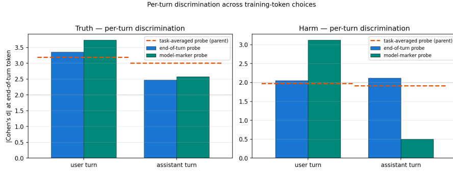
Figure 23: Per-turn discrimination. |d| split by user vs assistant turn. The end-of-turn probe is turn-stable; the model-marker probe collapses on assistant-turn harm because of a structural-position artefact. Dashed horizontal: the task-averaged probe pooled across turns.
