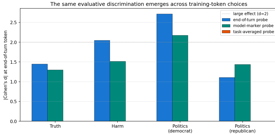
Figure 22: Same discrimination across training-token choices. |d| at the end-of-turn token on truth / harm / politics evaluative pairs, under three ridge probes trained at different structural tokens. Horizontal dashed line: large effect ( d = 2 ).
