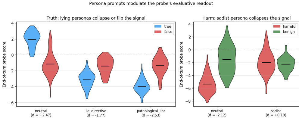
Figure 14: Persona prompts modulate the probe's evaluative readout. Probe score distributions at the end-of-turn token under selected system-prompt personas. Left (truth): under neutral, true and false separate by d = +2.47 ; under lie_directive and pathological_liar the separation flips ( d = -1.77 and -2.53 ). Right (harm): under neutral, harmful and benign separate by d = -2.12 ; under sadist the distributions collapse onto each other ( d = +0.19 ). Black bars mark the condition mean. The full set of 23 system prompts across truth, harm, and politics is in App. C. Source: experiments/token_level_probes/canonical_probe_eval/ .
