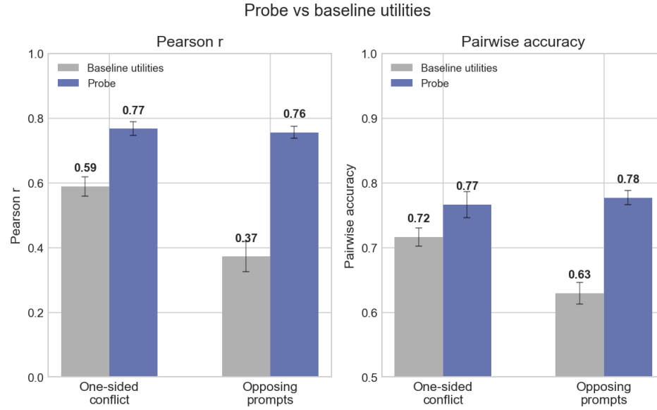
Figure 20: Re-fitted utilities under conflict prompts. Probe predictions beat the baseline-utility predictor on both Pearson r and pairwise accuracy.
