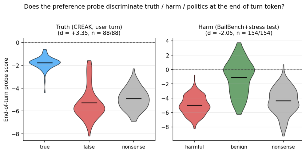
Figure 13: The preference probe separates truth and harm at the end-of-turn token. Violin plots of probe score by condition on paired evaluative stimuli under default conditions; black bar = mean. Nonsense condition (grey) sanity-checks that the effect is not driven by surprisal. Politics is omitted from this figure because the politics stimuli inherently include a system prompt; the partisan-prompt modulation story sits in Fig. 14. Source: experiments/token_level_probes/canonical_probe_eval/.
