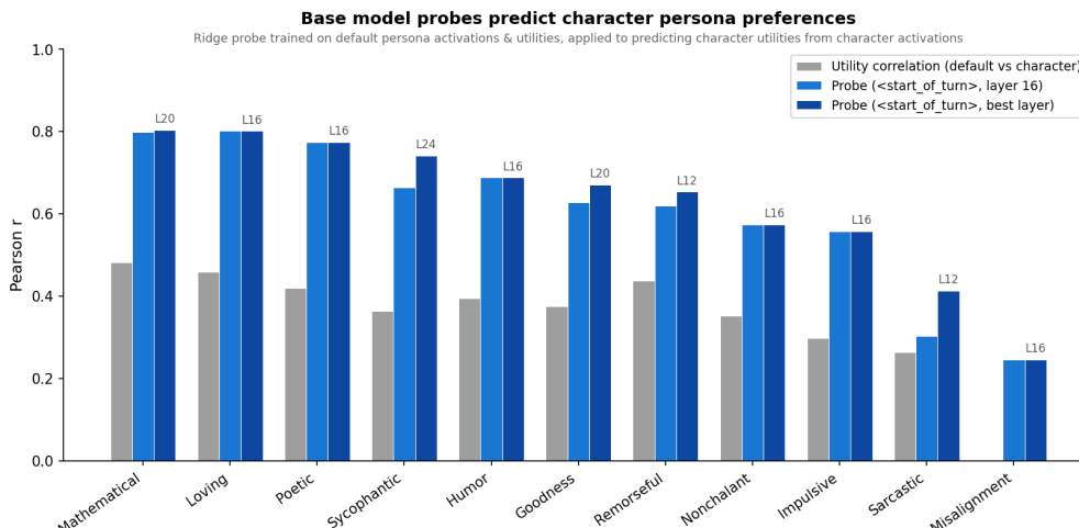
Figure 26: Base-model probe predicts character-fine-tuned persona preferences. Grey: raw correlation between base-model utilities and each character’s utilities. Light blue: probe at <start_of_turn>_2, layer 16. Dark blue: same selector, best layer per persona (layer annotated). The probe beats the utility-correlation baseline on 10/11 personas. Misalignment is the hardest case: its raw utilities anti-correlate with the base model ( r = -0.14 ), yet the probe still recovers a positive correlation ( r = 0.25 ) — the largest absolute gain of any persona.
