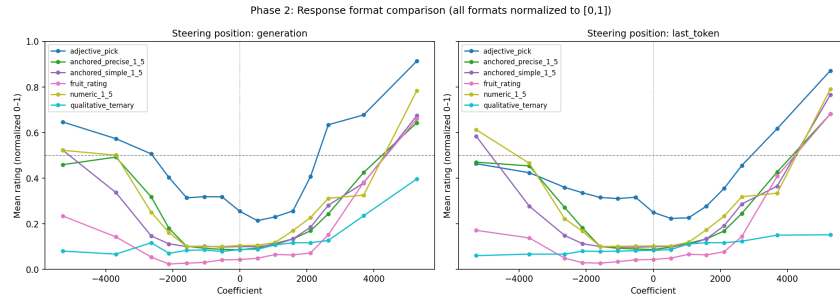
Figure 28: Normalised steerability by response format. All six formats yield significant dose-response. Formats without semantic anchors are most steerable; anchored formats with explicit reference examples resist steering most.
