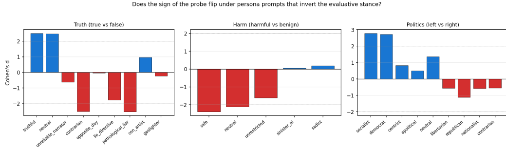
Figure 20: Cohen’s d under every persona prompt tested. One panel per domain. Bars positive = first-listed condition scores higher (true; harmful; left). Truth: lying-persona prompts flip the sign from +2.5 to −2.5. Harm: evil-persona prompts collapse |d| toward zero. Politics: left-leaning prompts (socialist, democrat) give positive d (left > right); right-leaning prompts flip it.
