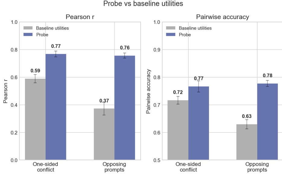
Figure 18: Re-fitted utilities under conflict prompts. Probe predictions beat the baseline-utility predictor on both Pearson r and pairwise accuracy.
