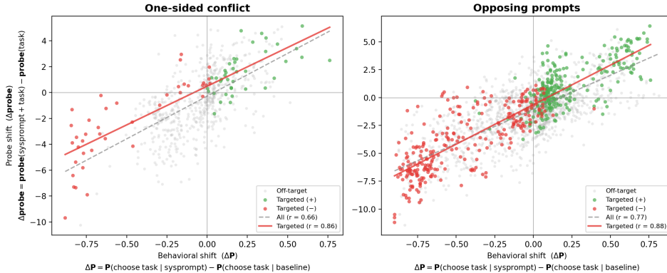
Figure 17: Probe delta vs behavioural delta on conflict/opposing prompts. One-sided conflict (left): r = 0.86 on targeted tasks. Opposing-pair prompts (right): r = 0.88 on targeted tasks.
