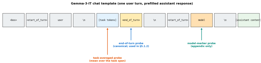
Figure 21: The three probe training positions in a Gemma-3-IT chat-formatted sequence. A typical user+assistant exchange tokenises to the row above. Coloured arrows mark the token where each probe is trained. All three probes are evaluated at the <end_of_turn> token in §5.1.2 and throughout this appendix.
