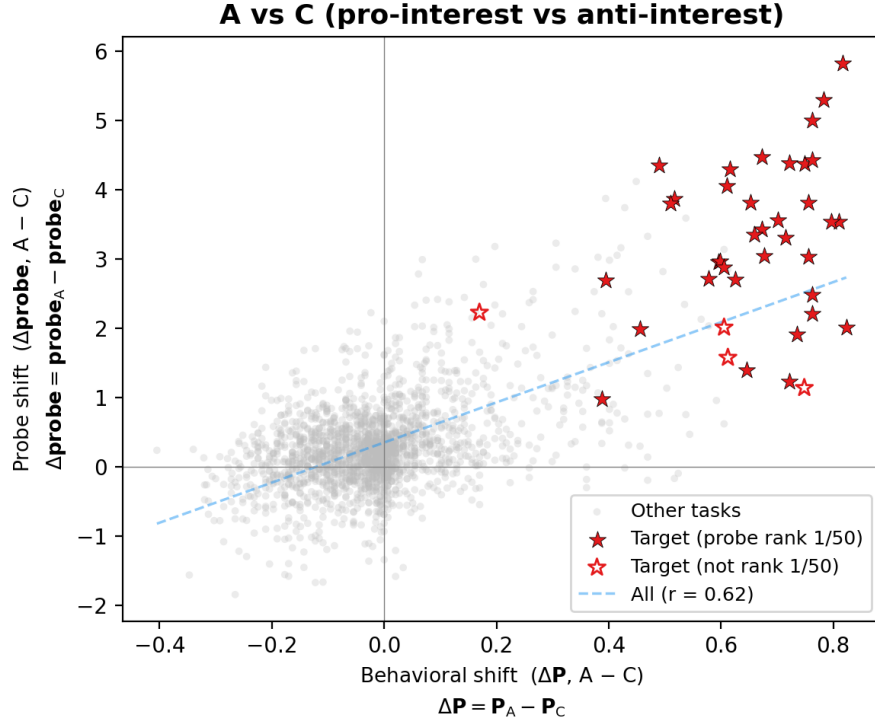
Figure 19: Fine-grained preference injection. Stars mark the target task for each biography; filled stars indicate the probe ranked it #1.
