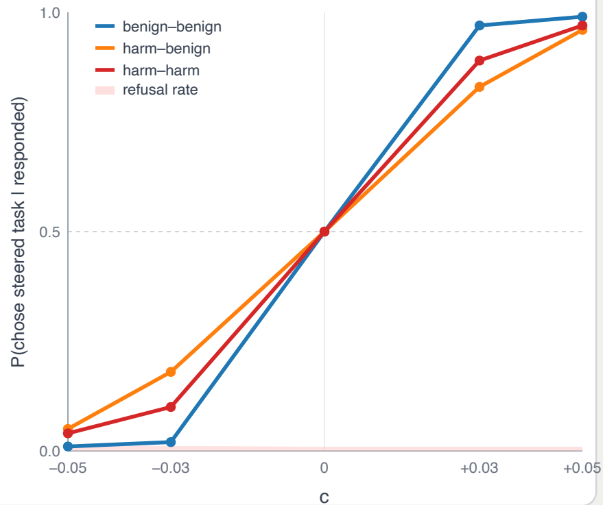
(a) Contrastive steering
