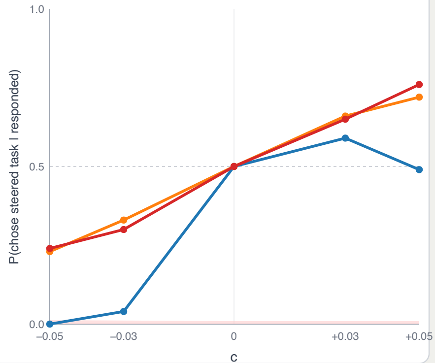
(b) Single-task steering
