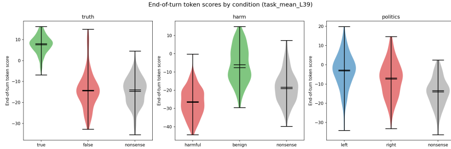
Figure 7: End-of-turn scores by evaluative condition. Applied at the end-of-turn token, the preference probe separates true vs false, harmful vs benign, and left vs right conditions by d \approx 2-3 . Source: experiments/token_level_probes/ .
