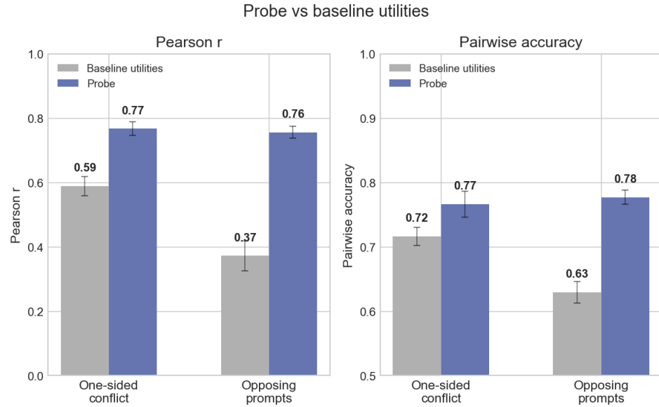
Figure 15: Re-fitted utilities under conflict prompts. Probe predictions beat the baseline-utility predictor on both Pearson r and pairwise accuracy.
