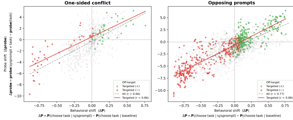
Figure 14: Probe delta vs behavioural delta on conflict/opposing prompts. One-sided conflict (left): r = 0.86 on targeted tasks. Opposing-pair prompts (right): r = 0.88 on targeted tasks.
