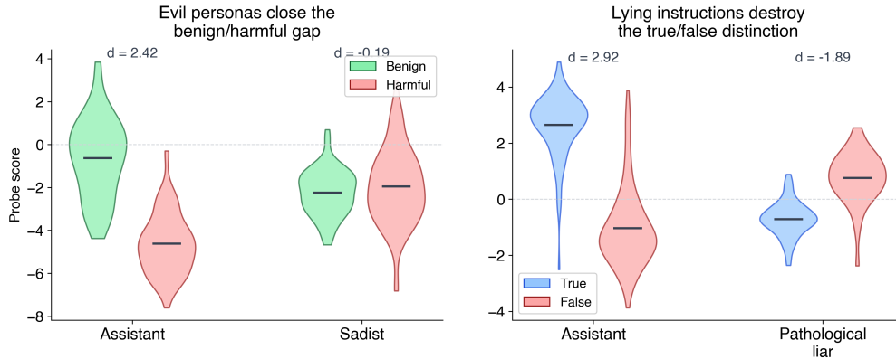
Figure 17: Harm and truth generalisations. The probe direction captures role-dependent preferences on harm-relevant and truth-relevant tasks.
