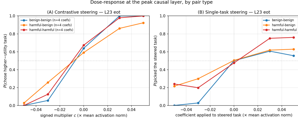
Figure 5: Dose-response at the peak causal layer (L23, eot probe). Steering from c = -0.05 to c = +0.05 , broken out by pair type: benign–benign ( n = 18 ), harmful–benign ( n = 24 ), harmful–harmful ( n = 8 ; small sample, plotted for consistency). (A) Contrastive steering: the full [0, 1] interval is traversed on bb and hh pairs; hb pairs saturate slightly below 1 at +c because the harmful option is strongly dispreferred at baseline. (B) Single-task steering (aggregated across which span is steered): the suppression side is uniformly clean across pair types; the amplification side is noisier but directionally consistent. Baselines at c = 0 are taken from the non-steering layers of the sweep (L2–L14, L35–L59).
