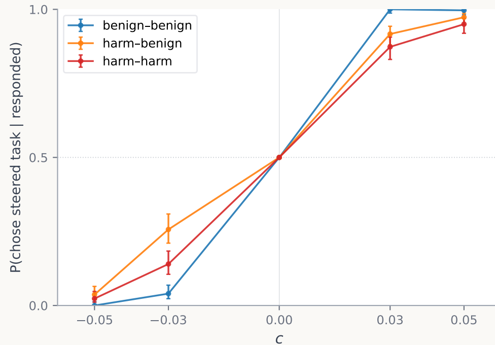
(a) Contrastive steering
