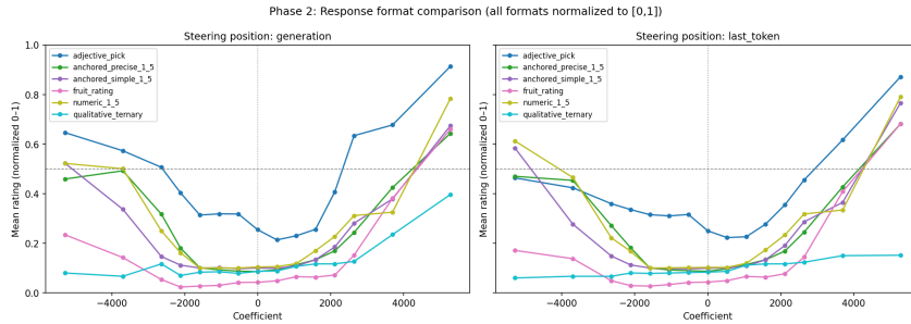
Figure 26: Normalised steerability by response format. All six formats yield significant dose-response. Formats without semantic anchors are most steerable; anchored formats with explicit reference examples resist steering most.
