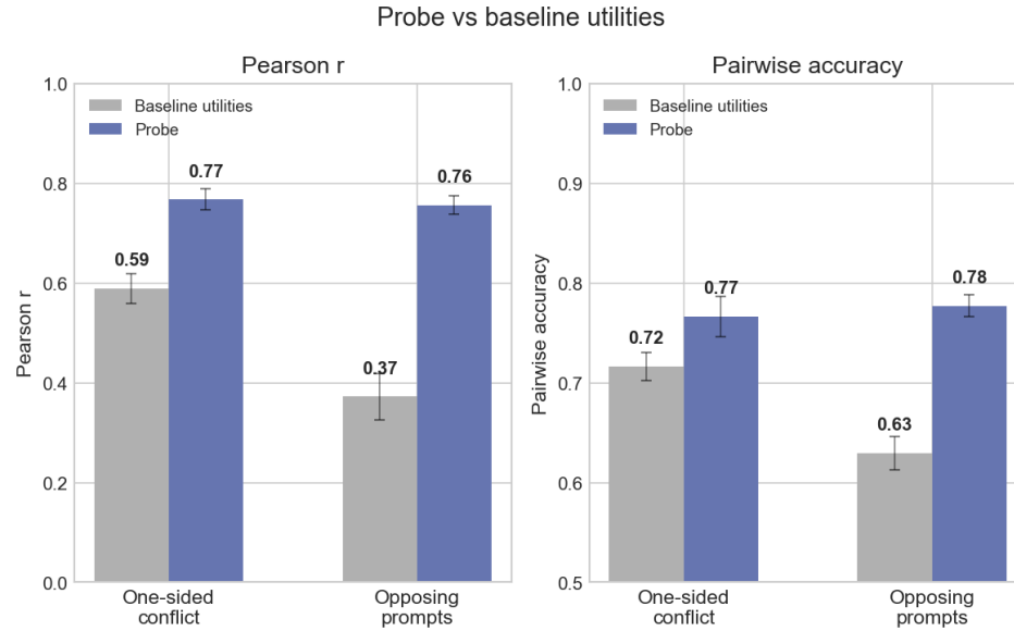
Figure 15: Re-fitted utilities under conflict prompts. Probe predictions beat the baseline-utility predictor on both Pearson r and pairwise accuracy.
