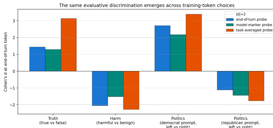
Figure 27: Same discrimination across training-token choices. Cohen’s d at the end-of-turn token on truth / harm / politics evaluative pairs, under three ridge probes trained at the different structural tokens marked in Fig. 26. Positive = first-listed class scores higher (true; harmful; left). All three probes agree in sign; democrat-prompt politics is positive, republican-prompt politics flips negative.
