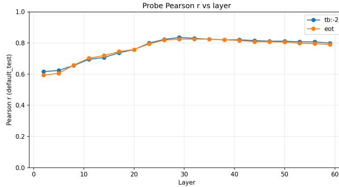
Figure 18: Held-out Pearson r of ridge probes fit at 20 layers spanning 3–95% depth. Two selectors: the final prompt (turn-boundary, tb:-2) and end-of-turn (eot) token. Both rise steeply through mid-network, peak in a broad plateau at L26–L35, and decline slowly to L59. Peak r = 0.835 at L29 (tb:-2); 0.825 at L32 (eot). The two selectors are nearly indistinguishable in the plateau — token choice barely matters in the readable region.
