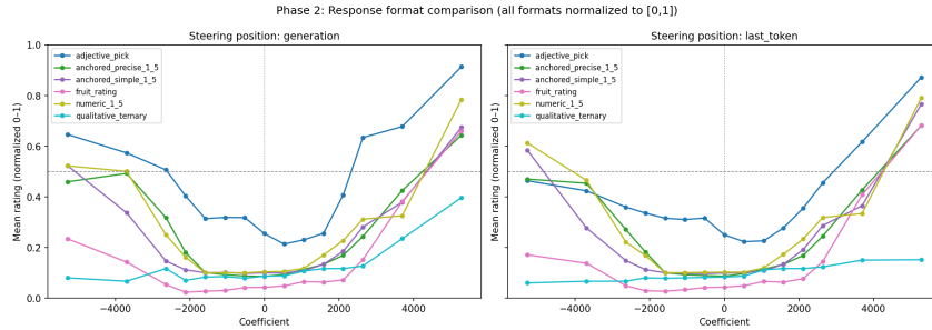
Figure 38: Normalised steerability by response format. All six formats yield significant dose-response. Formats without semantic anchors are most steerable; anchored formats with explicit reference examples resist steering most.
