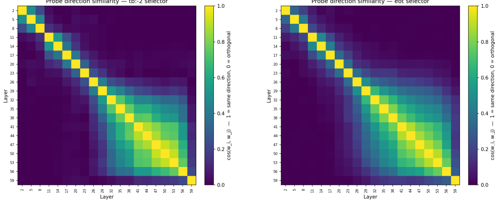
Figure 19: Within-selector probe-direction cosine. Left: tb:-2; right: eot. Both selectors show the same block structure: early layers (L2–L17) and late layers (L29–L59) form two loosely-aligned families, with the late block mutually aligned at cosine \geq 0.5 and internally tightly aligned ( \geq 0.8 ) among adjacent layers. Early layers are close to orthogonal to the late block.
