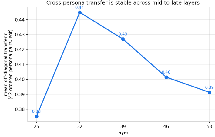
Figure 31: Mean off-diagonal transfer r across layers (eot). Average over all 42 ordered (train, eval) persona pairs. The cross-persona transfer signal is approximately layer-invariant in the L25–L53 range.
