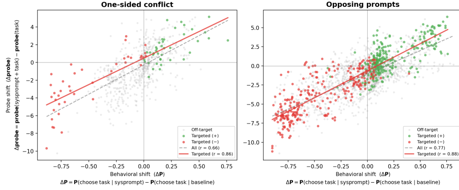
Figure 22: Probe delta vs behavioural delta on conflict/opposing prompts. One-sided conflict (left): r = 0.86 on targeted tasks. Opposing-pair prompts (right): r = 0.88 on targeted tasks.
