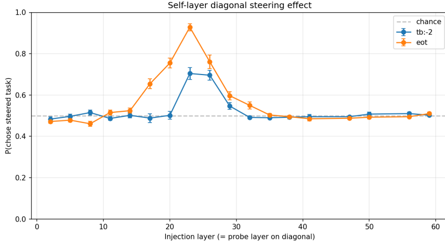
Figure 5: Intervention-site sweep. Self-layer contrastive steering (probe trained at L, injected at L) at |c| = 0.05 . Preference swing rises sharply from L17, peaks at L23, and collapses above L35. The tb:-2 and eot token-position variants of the probe trace the same profile; eot gives a stronger peak. Layers L17–L26 define the causal window.
