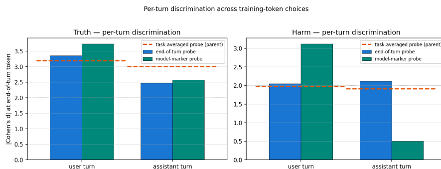
Figure 28: Per-turn discrimination. |d| split by user vs assistant turn. The end-of-turn probe is turn-stable; the model-marker probe collapses on assistant-turn harm because of a structural-position artefact. Dashed horizontal: the task-averaged probe pooled across turns.
