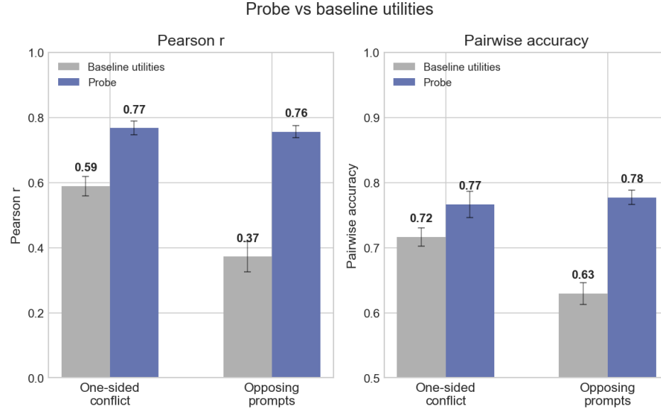
Figure 23: Re-fitted utilities under conflict prompts. Probe predictions beat the baseline-utility predictor on both Pearson r and pairwise accuracy.
