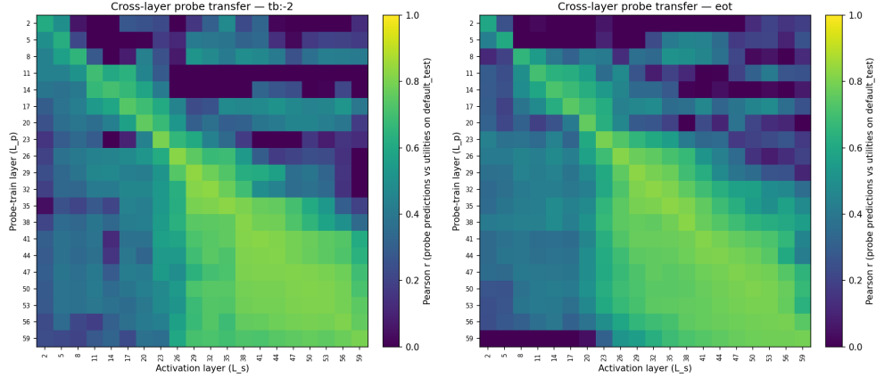
Figure 21: Cross-layer probe transfer. Each cell: Pearson r between predictions of the probe trained at layer L_p (row) evaluated on activations at layer L_s (column), versus held-out utilities. The diagonal is each probe’s native performance (equivalent to Fig. 18). Off-diagonal cells in the mid-to-late block stay near the diagonal value, reflecting the tight cosine alignment seen in Fig. 19. Early-layer probes (top rows) transfer poorly to late activations and vice versa.
