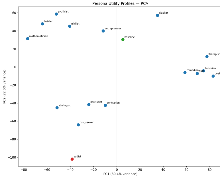
Figure 30: PCA of the 16-persona utility sweep. Each point is a persona’s Thurstonian utility profile on the 500-task stratified sample, projected onto the first two principal components (52% of variance). Three clusters emerge: structured/analytical (left), creative/humanistic (right), dark/oppositional (bottom-centre). Sadist (red) is the only persona whose utility anti-correlates with the no-system-prompt baseline (green). The final six-persona set takes one representative per cluster plus sadist, slacker, and aura.
