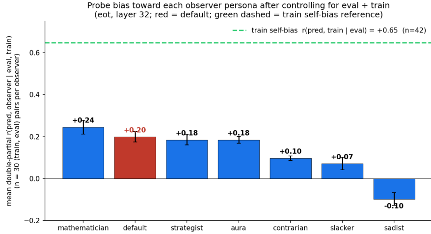
Figure 35: Probe bias toward each observer persona after controlling for eval and train. Mean double-partial r(\hat{u}, u_X \mid u_E, u_T) across 30 ordered (T, E) pairs per observer; error bars are SEM. Green dashed line: train self-bias r(\hat{u}, u_T \mid u_E) = +0.648 (42 pairs). Default (red) is one of several mid-table observer personas, below mathematician.
