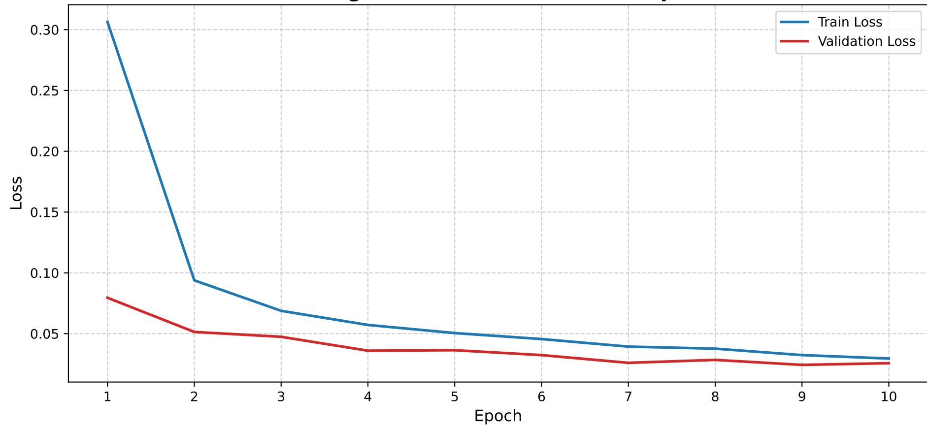
Training & Validation Loss Over Epochs
