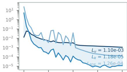
Loss
