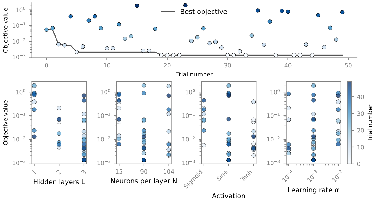
MLP, Infinite, Best trial 19, (L, N, \sigma , \alpha )=(3, 90, Sine, 1e-03) and Objective value=1.3e-03
