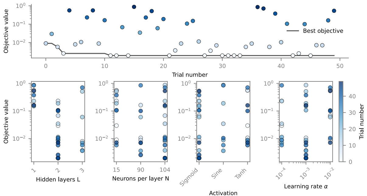
MLP, Semi-infinite, Best trial 11, (L, N, \sigma , \alpha )=(2, 104, Sigmoid, 1e-03) and Objective value=2.0e-03
