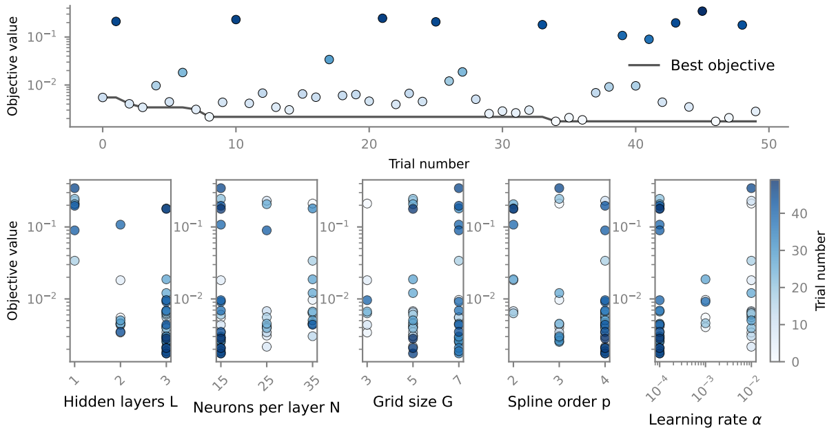
KAN, Infinite, Best trial 46, (L, N, G, p, \alpha )=(3, 15, 5, 4, 1e-04) and Objective value=1.7e-03
