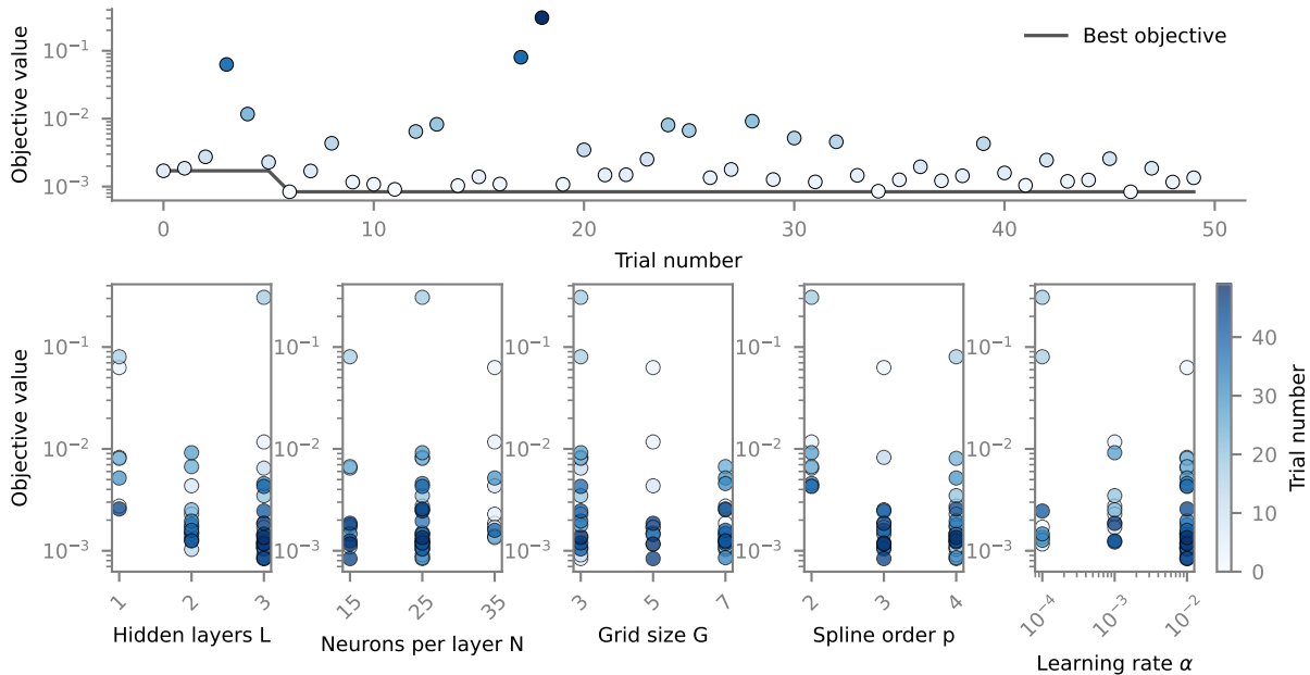
KAN, Semi-infinite, Best trial 46, (L, N, G, p, \alpha )=(3, 15, 5, 3, 1e-02) and Objective value=8.4e-04
