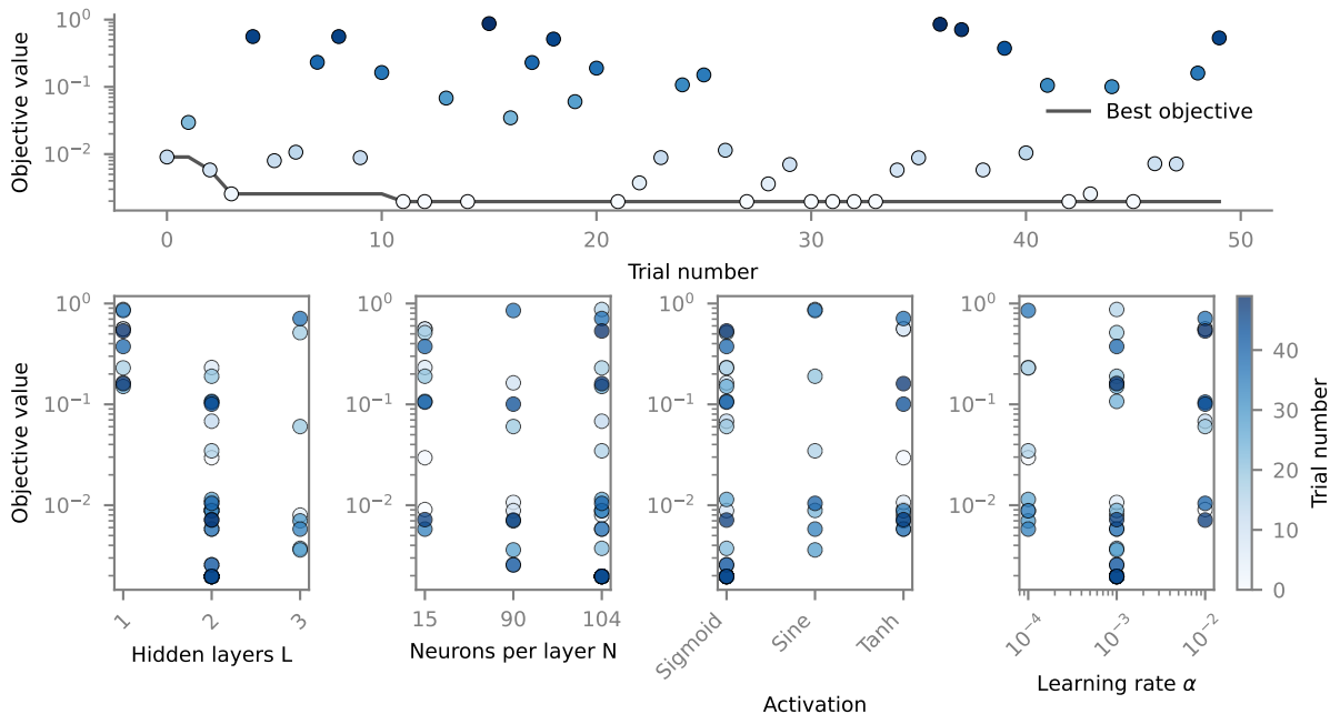
MLP, Semi-infinite, Best trial 11, (L, N, \sigma, \alpha)=(2, 104, \text{Sigmoid}, 1\text{e-}03) and Objective value= 2.0\text{e-}03
