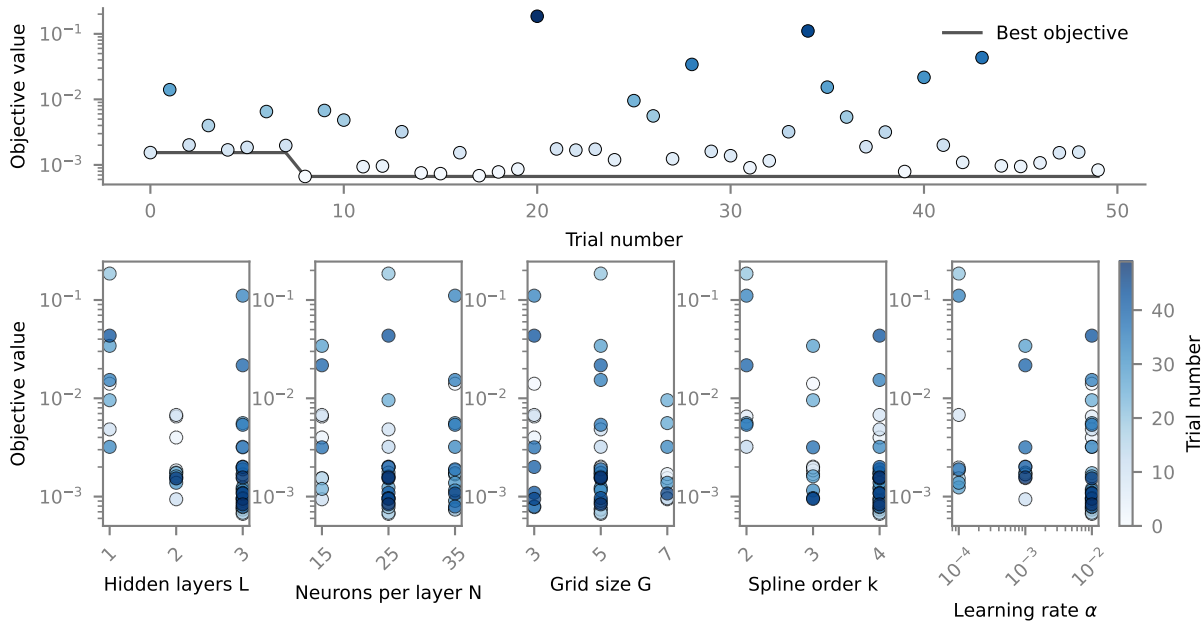
KAN, Semi-infinite, Best trial 8, (L, N, G, k, \alpha )=(3, 25, 5, 4, 1e-02) and Objective value=6.7e-04
