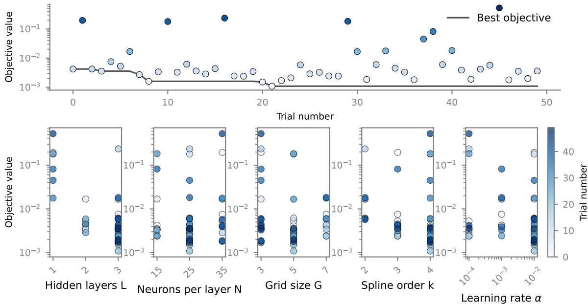
KAN, Infinite, Best trial 21, (L, N, G, k, \alpha )=(3, 25, 5, 4, 1e-02) and Objective value=1.1e-03
