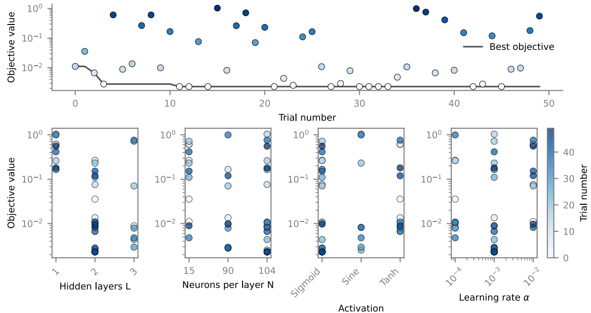
MLP, Semi-infinite, Best trial 11, (L, N, G, k, \alpha )=(2, 104, Sigmoid, 1e-03) and Objective value=2.3e-03
