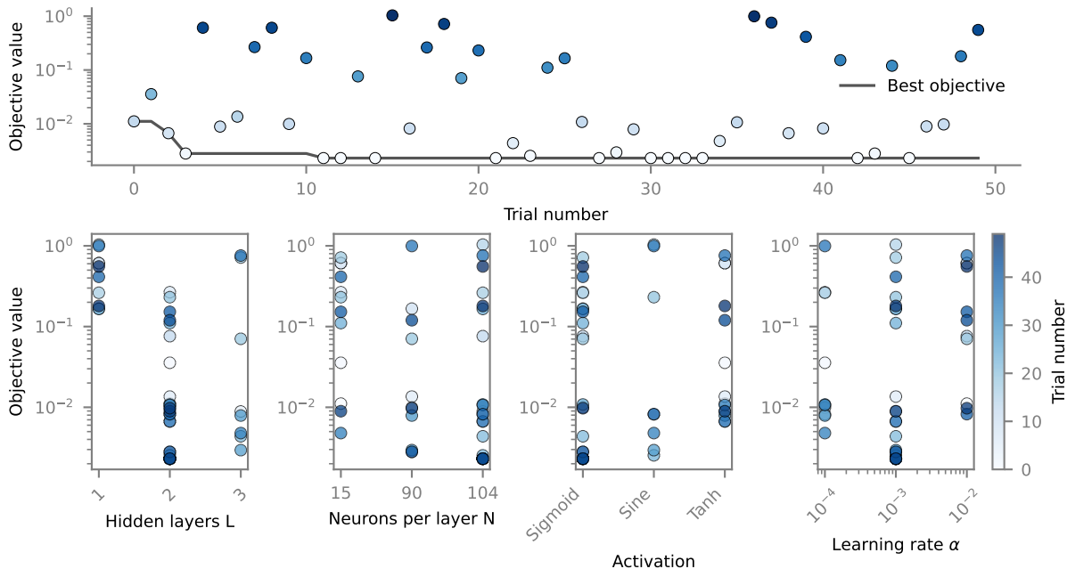
MLP, Semi-infinite, Best trial 11, (L, N, G, k, \alpha)=(2, 104, \text{Sigmoid}, 1e-03) and Objective value= 2.3e-03
