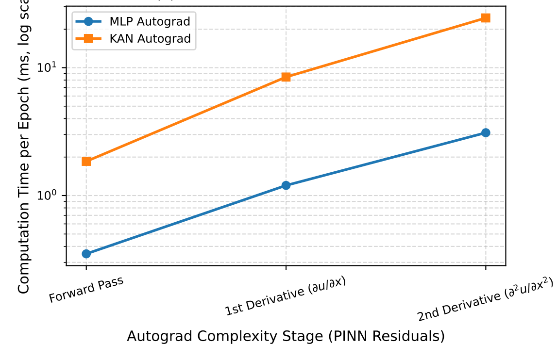
(c) Automatic Differentiation Cost
