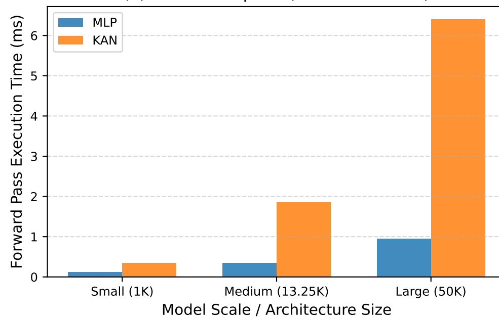
(b) Inference Speed (Wall-Clock Time)
