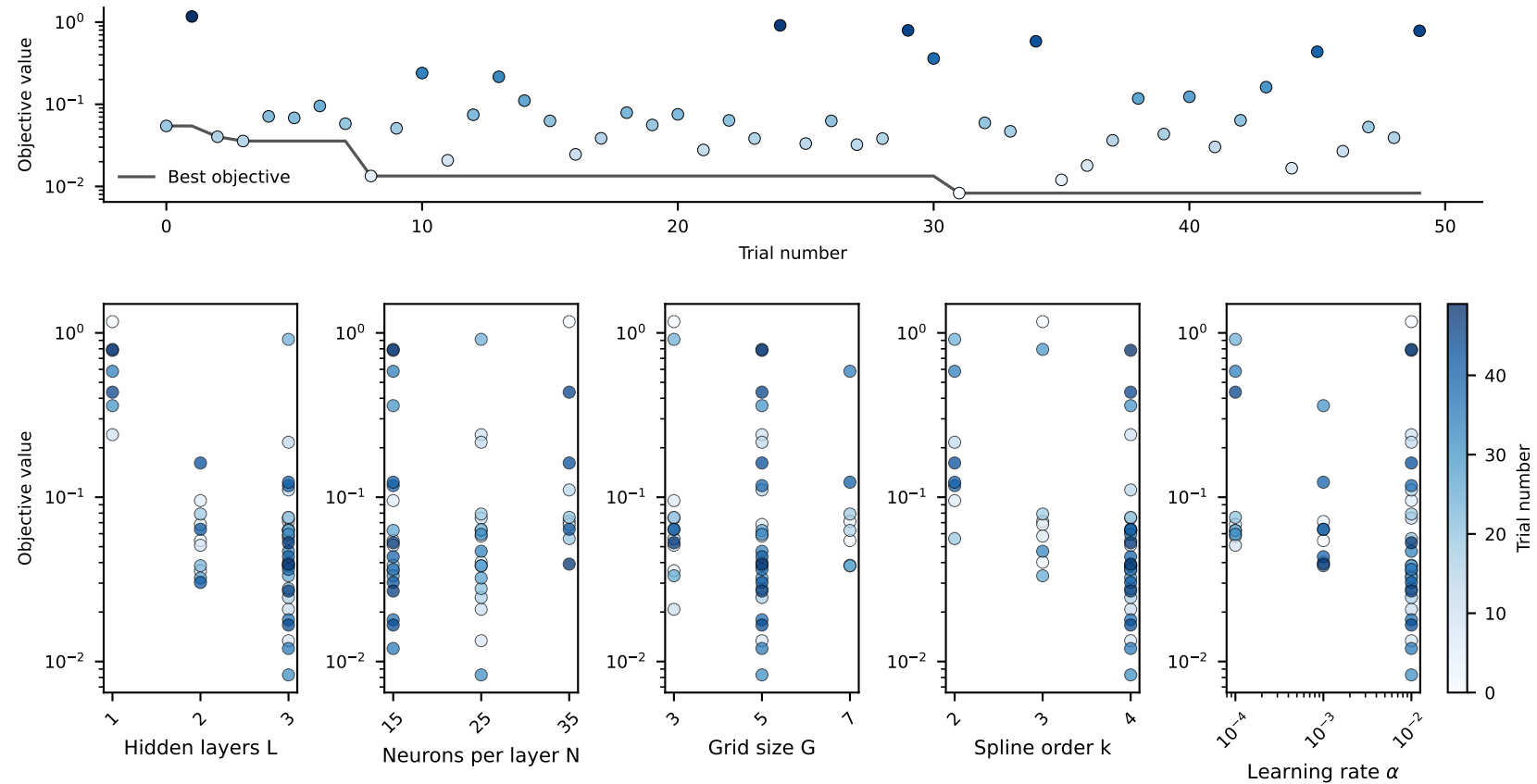
KAN, Semi-infinite, Best trial 31, (L, N, G, k, \alpha )=(3,25,5,4,1e-02) and Objective value=8.3e-03
