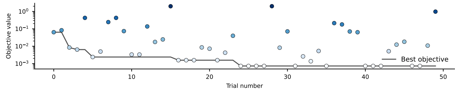
MLP, Infinite, Best trial 24, (L, N, G, k, \alpha )=(3,90,Sine,1e-03) and Objective value=7.3e-04
