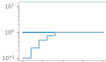
\lambda_{\text{PDE}} schedule
