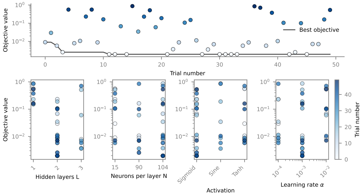
MLP, Semi-infinite, Best trial 11, (L, N, G, k, \alpha)=(2, 104, \text{Sigmoid}, 1e-03) and Objective value= 2.0e-03
