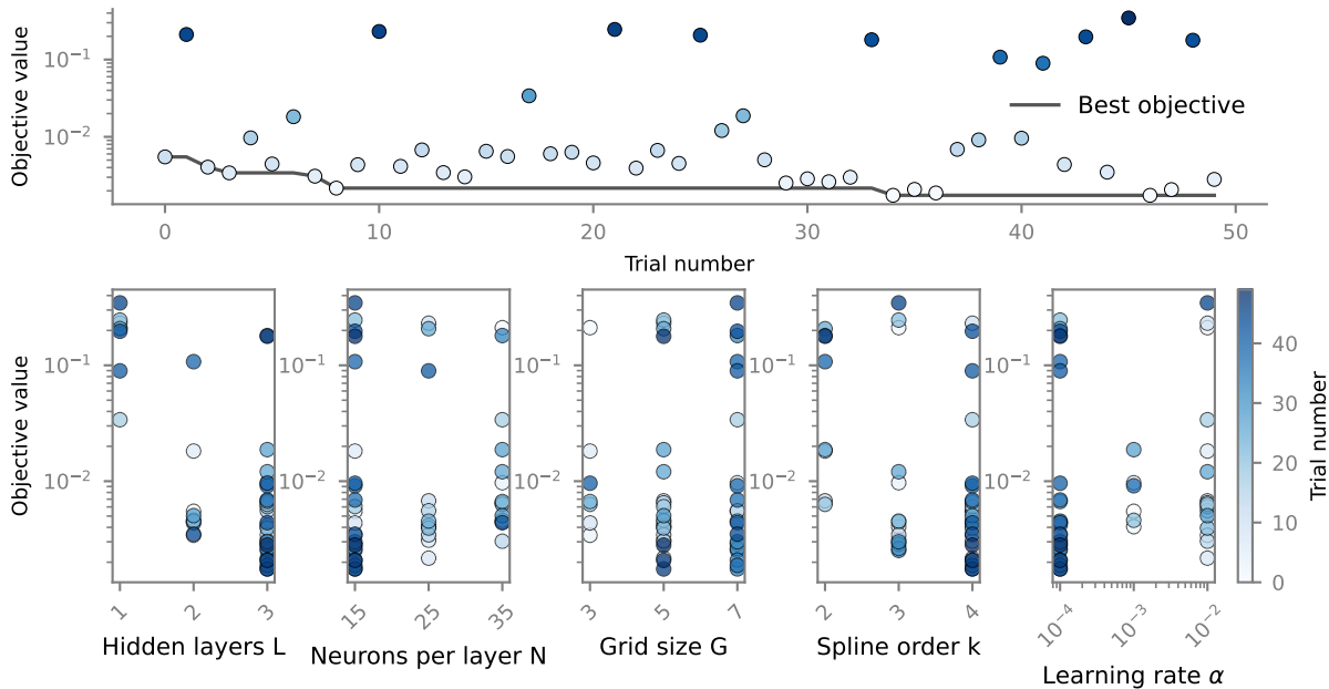
KAN, Infinite, Best trial 46, (L, N, G, k, \alpha )=(3, 15, 5, 4, 1e-04) and Objective value=1.7e-03
