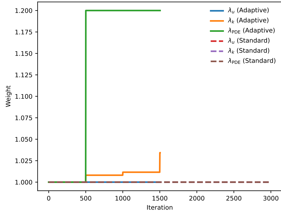
Loss weights
