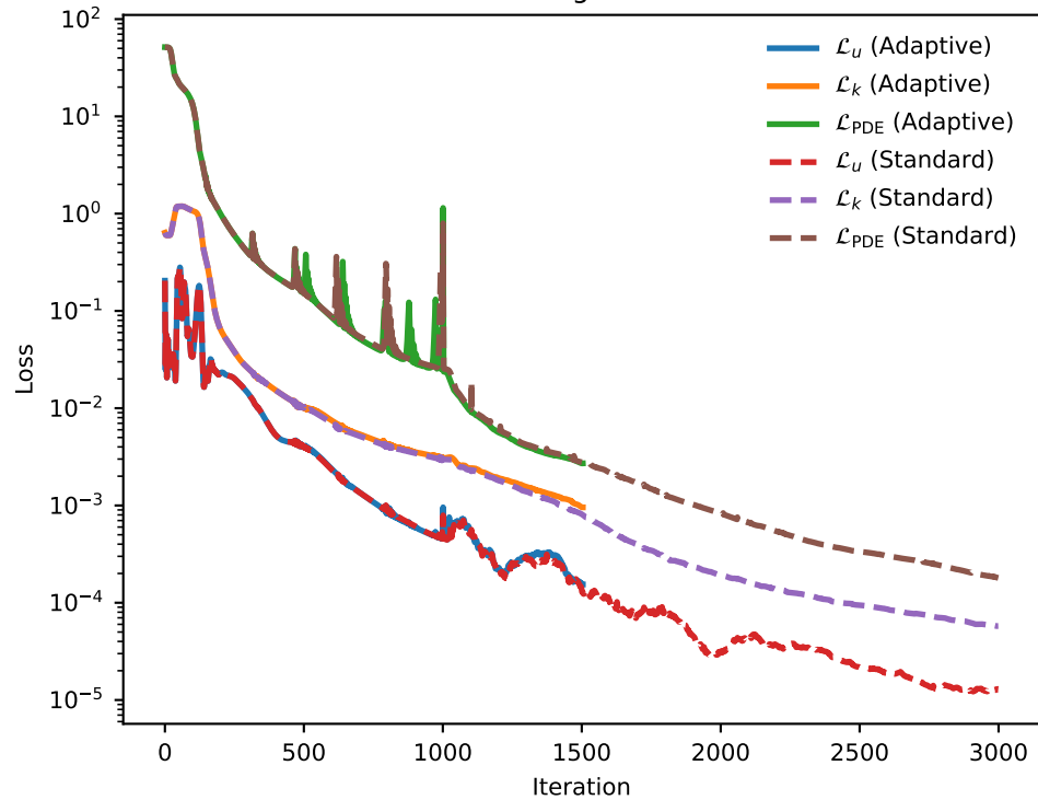
Training losses
