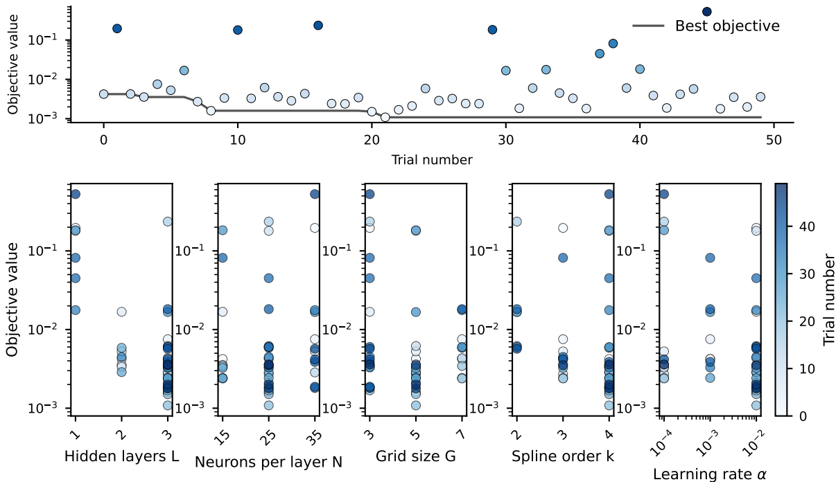
KAN, Infinite, Best trial 21, (L, N, G, k, \alpha )=(3,25,5,4,1e-02) and Objective value=1.1e-03
