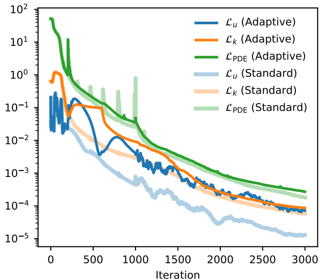
Loss
