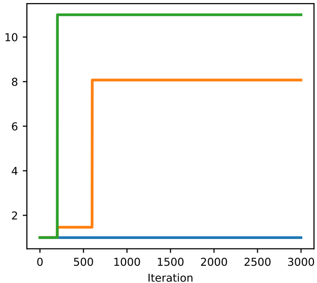
Weight
