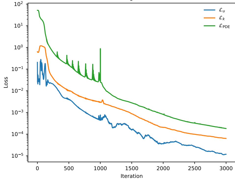
Training losses
