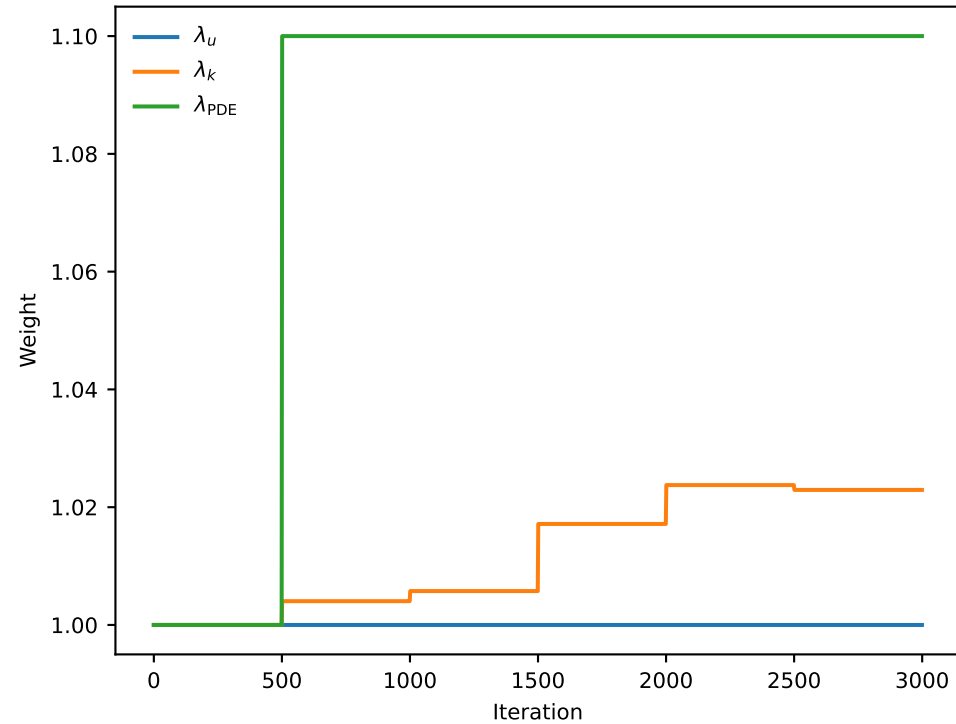
Adaptive weights
