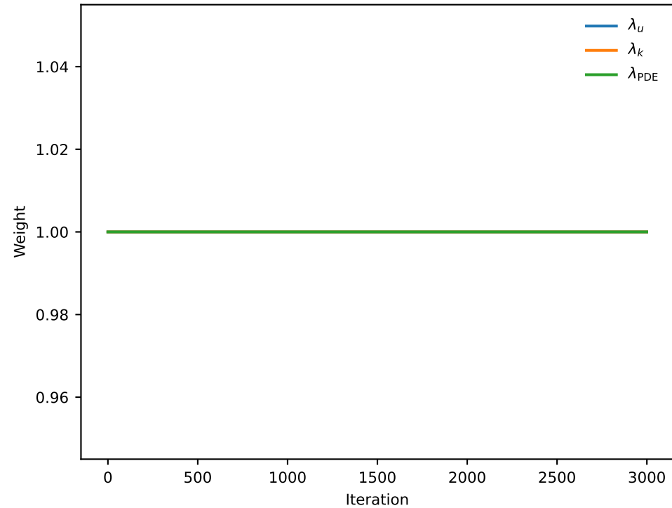
Adaptive weights
