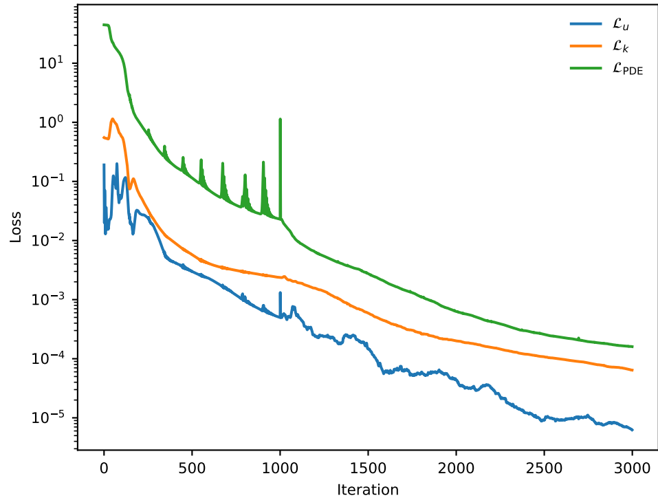
Training losses
