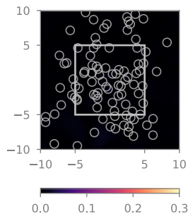
Gaussian
